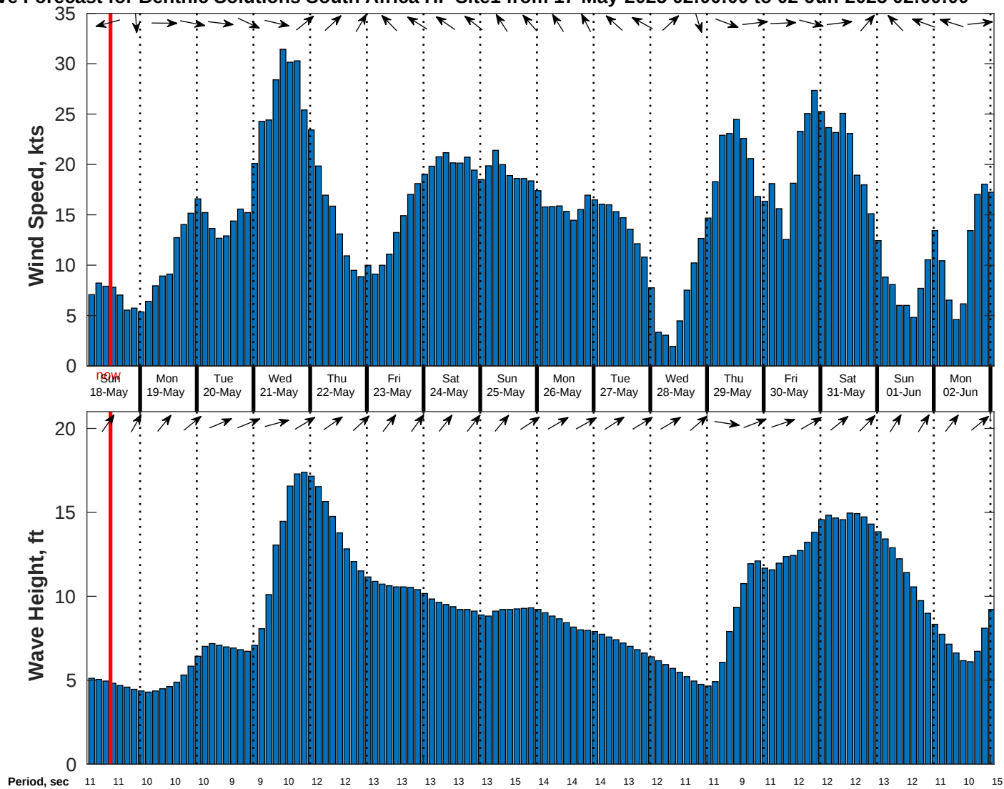
Wind & Wave Forecast for Benthic Solutions South Africa HF Site1 from 17-May-2025 02:00:00 to 02-Jun-2025 02:00:00
