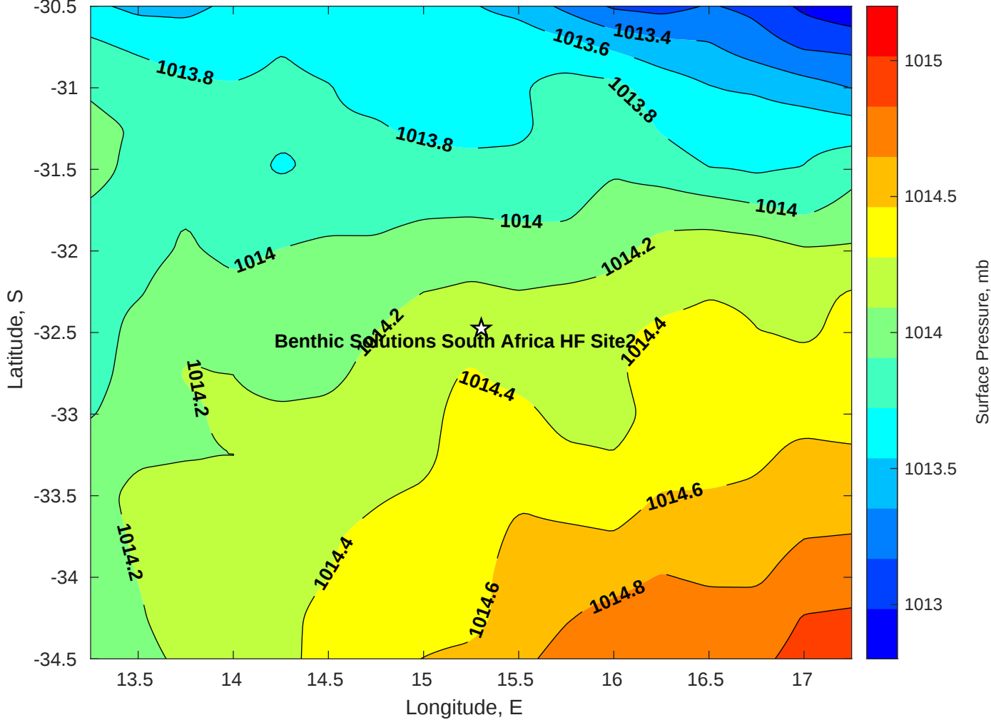
Surface Pressure (mb) for Benthic Solutions South Africa HF Site2 at 17-May-2025 00:00:00
