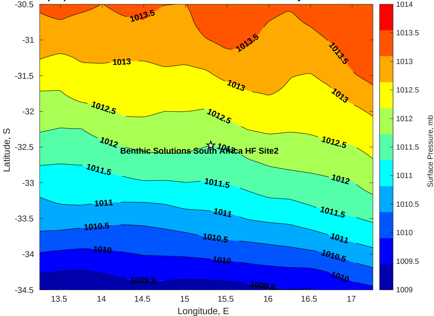
Surface Pressure (mb) for Benthic Solutions South Africa HF Site2 at 19-May-2025 00:00:00
