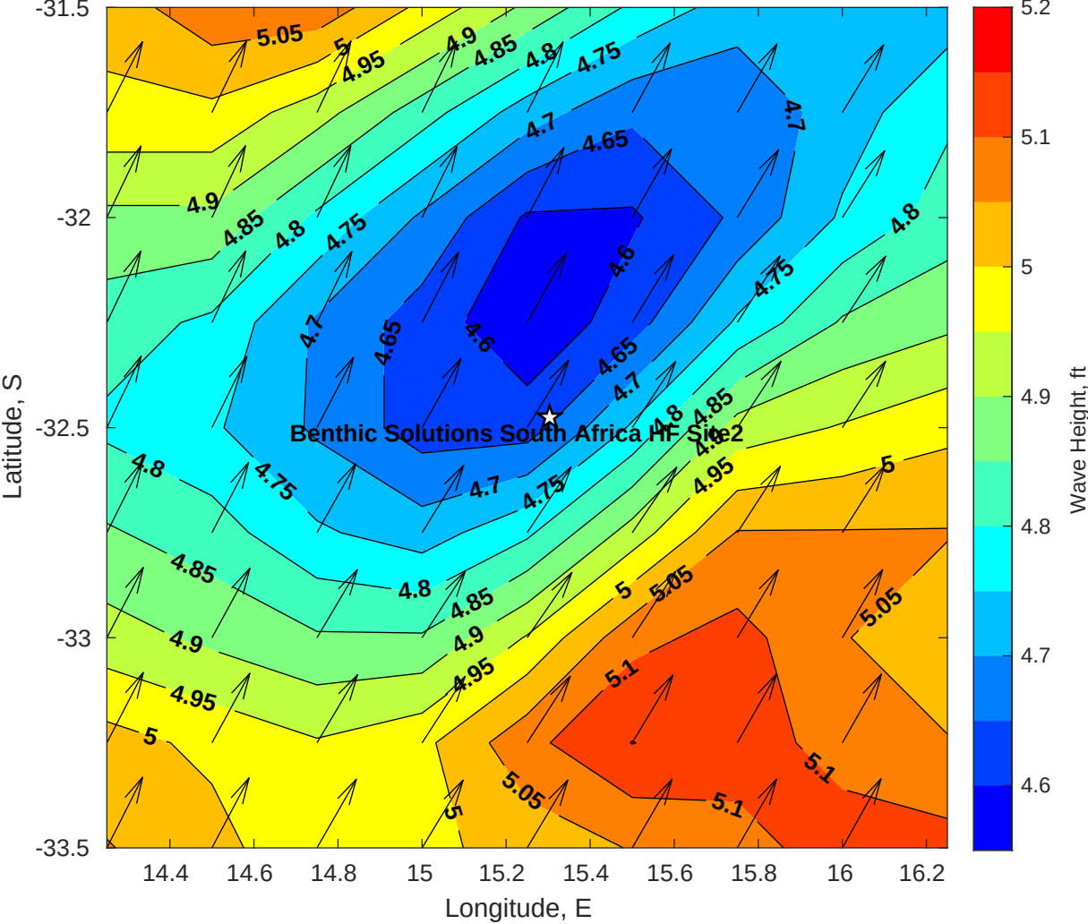
Wave Height (ft) for Benthic Solutions South Africa HF Site2 at 17-May-2025 09:00:00
