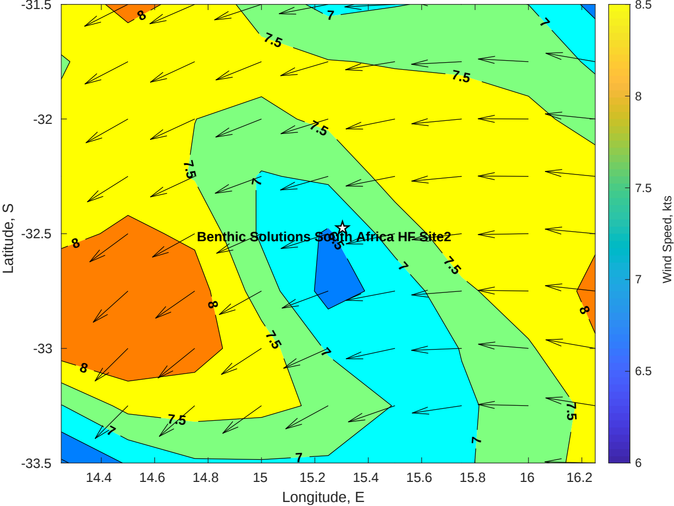
Winds (kts) for Benthic Solutions South Africa HF Site2 at 17-May-2025 09:00:00
