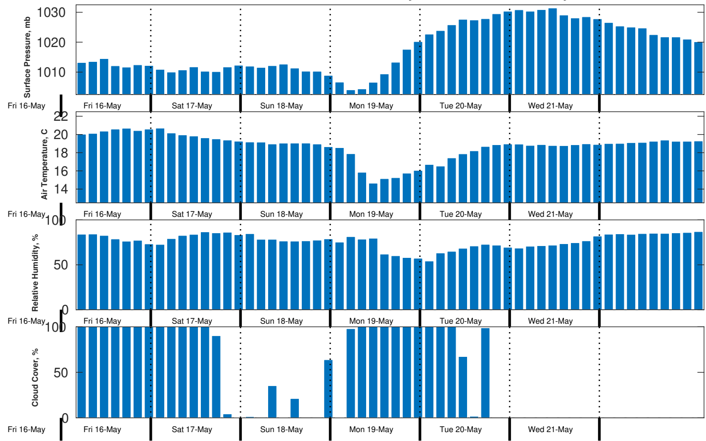
Met Forecast for Benthic Solutions South Africa HF Site2 from 17-May-2025 00:00:00 to 24-May-2025 00:00:00
