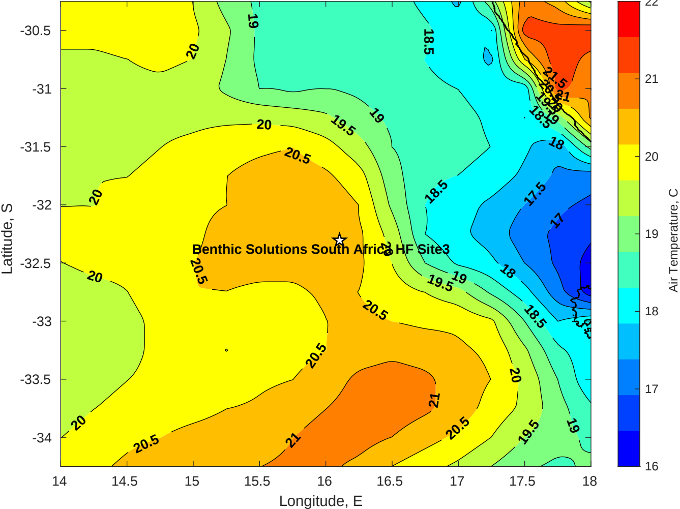
Air Temperature (C) for Benthic Solutions South Africa HF Site3 at 17-May-2025
