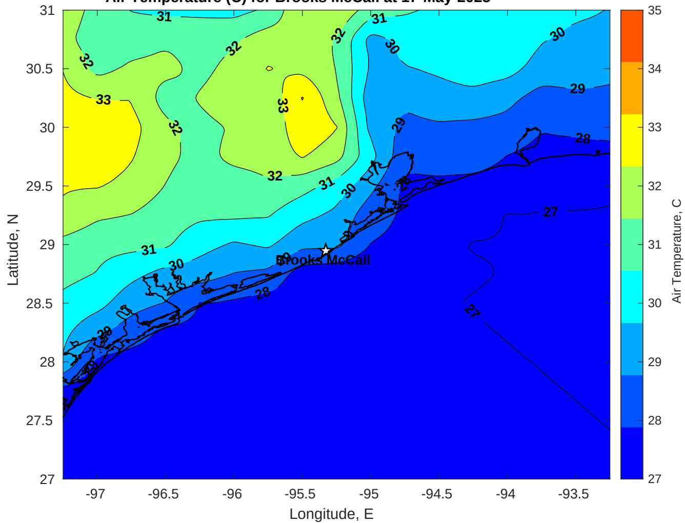
Air Temperature (C) for Brooks McCall at 17-May-2025
