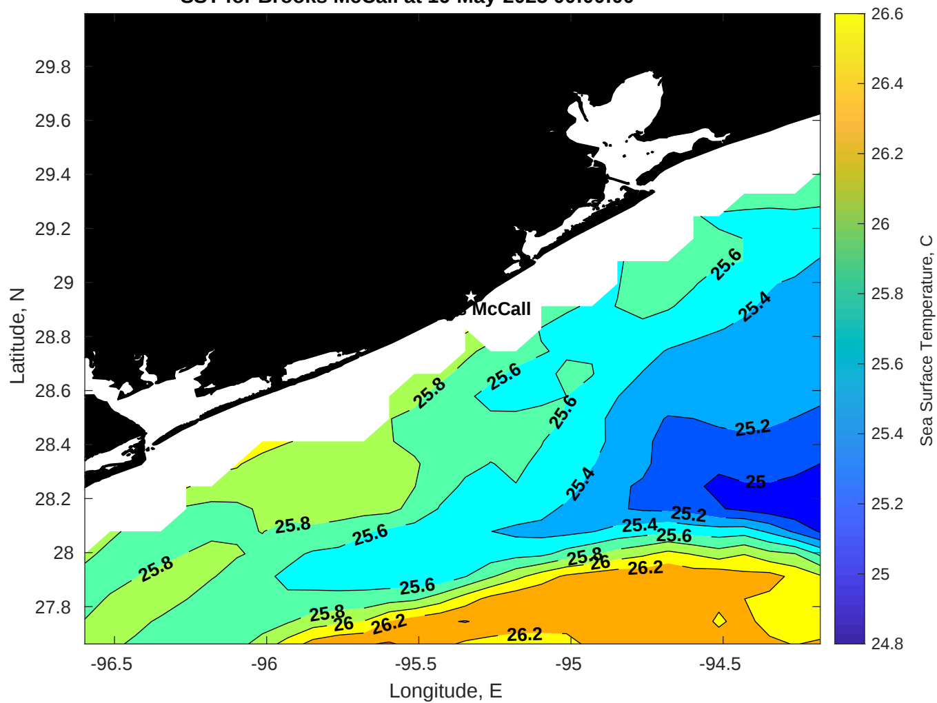
SST for Brooks McCall at 16-May-2025 00:00:00
