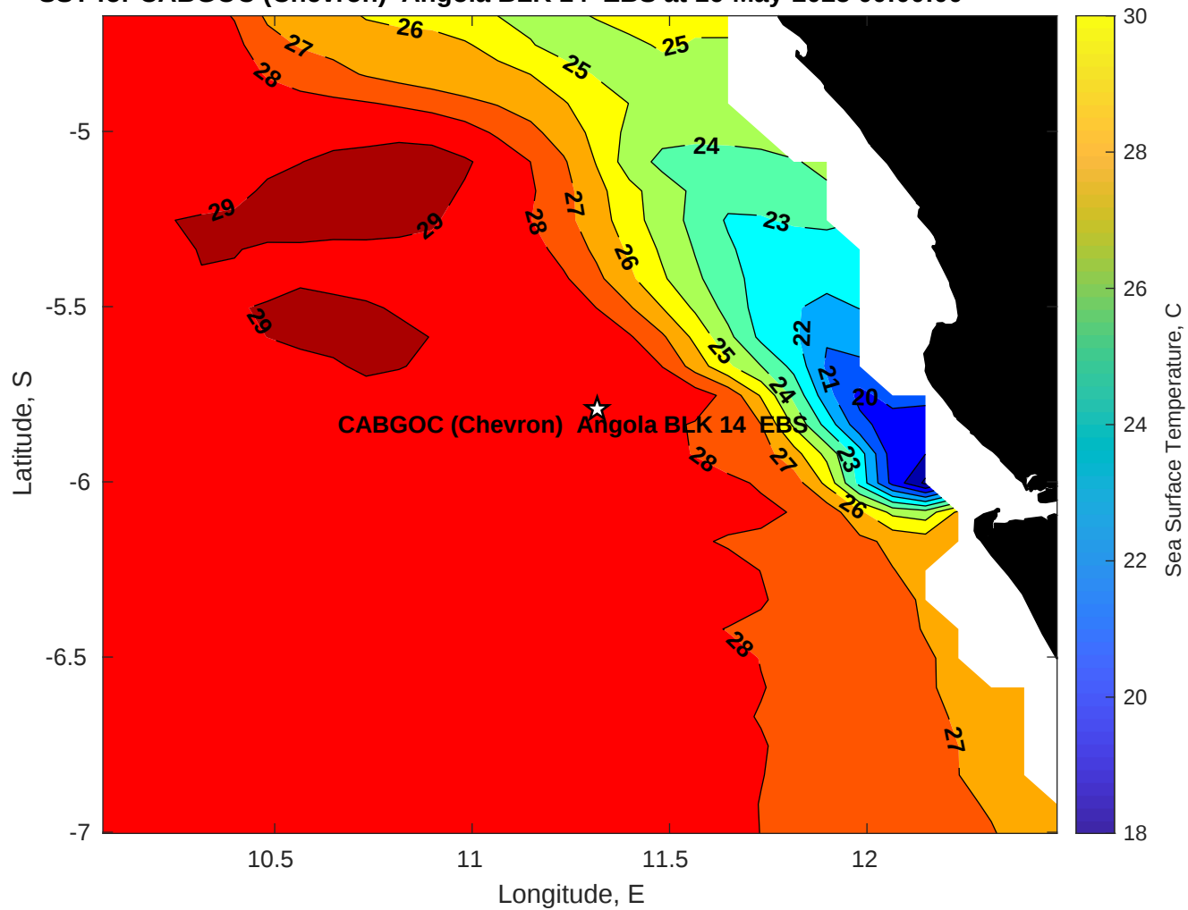
SST for CABGOC (Chevron) Angola BLK 14 EBS at 16-May-2025 00:00:00
