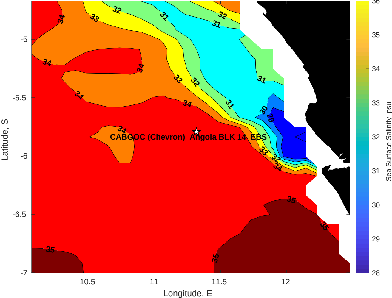
Surface Salinity for CABGOC (Chevron) Angola BLK 14 EBS at 16-May-2025 00:00:00
