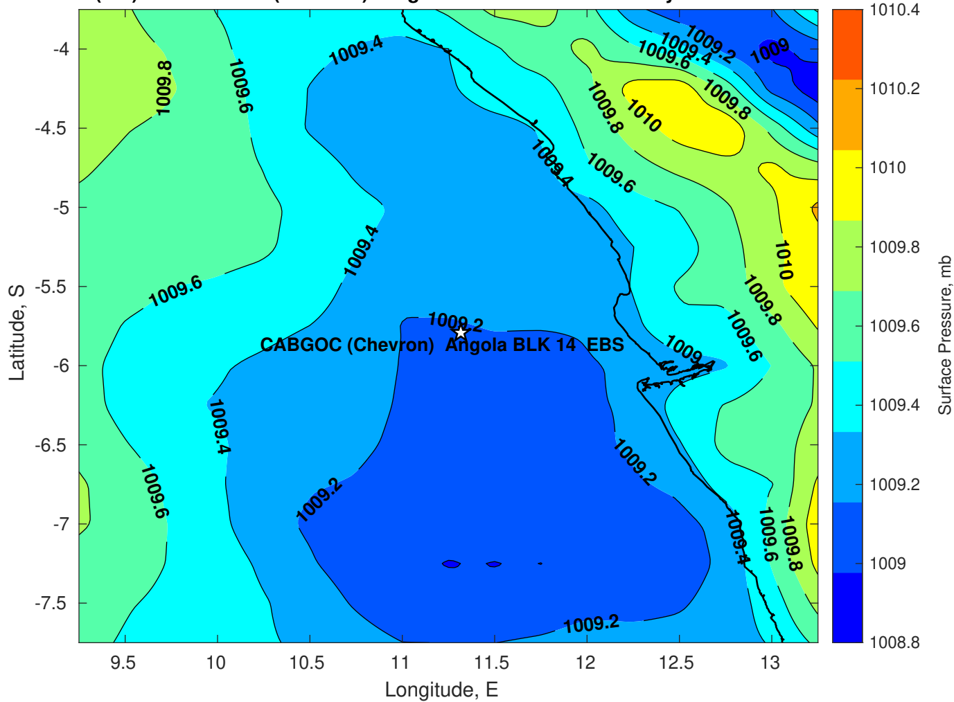
Surface Pressure (mb) for CABGOC (Chevron) Angola BLK 14 EBS at 18-May-2025 00:00:00
