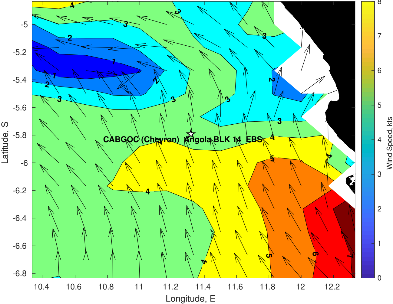
Winds (kts) for CABGOC (Chevron) Angola BLK 14 EBS at 17-May-2025 09:00:00
