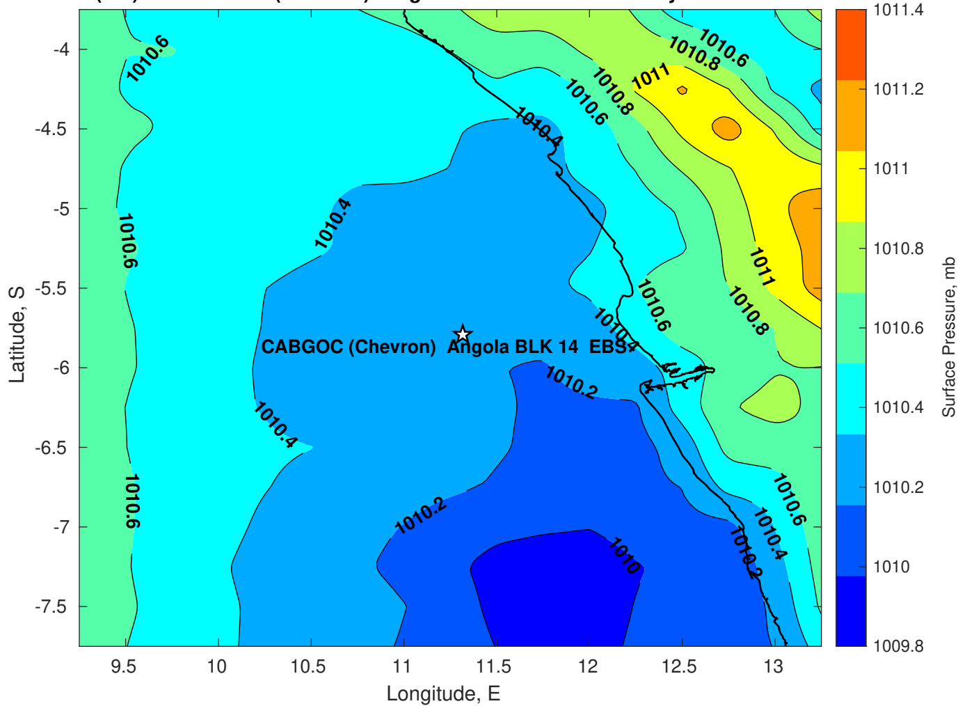
Surface Pressure (mb) for CABGOC (Chevron) Angola BLK 14 EBS at 19-May-2025 00:00:00
