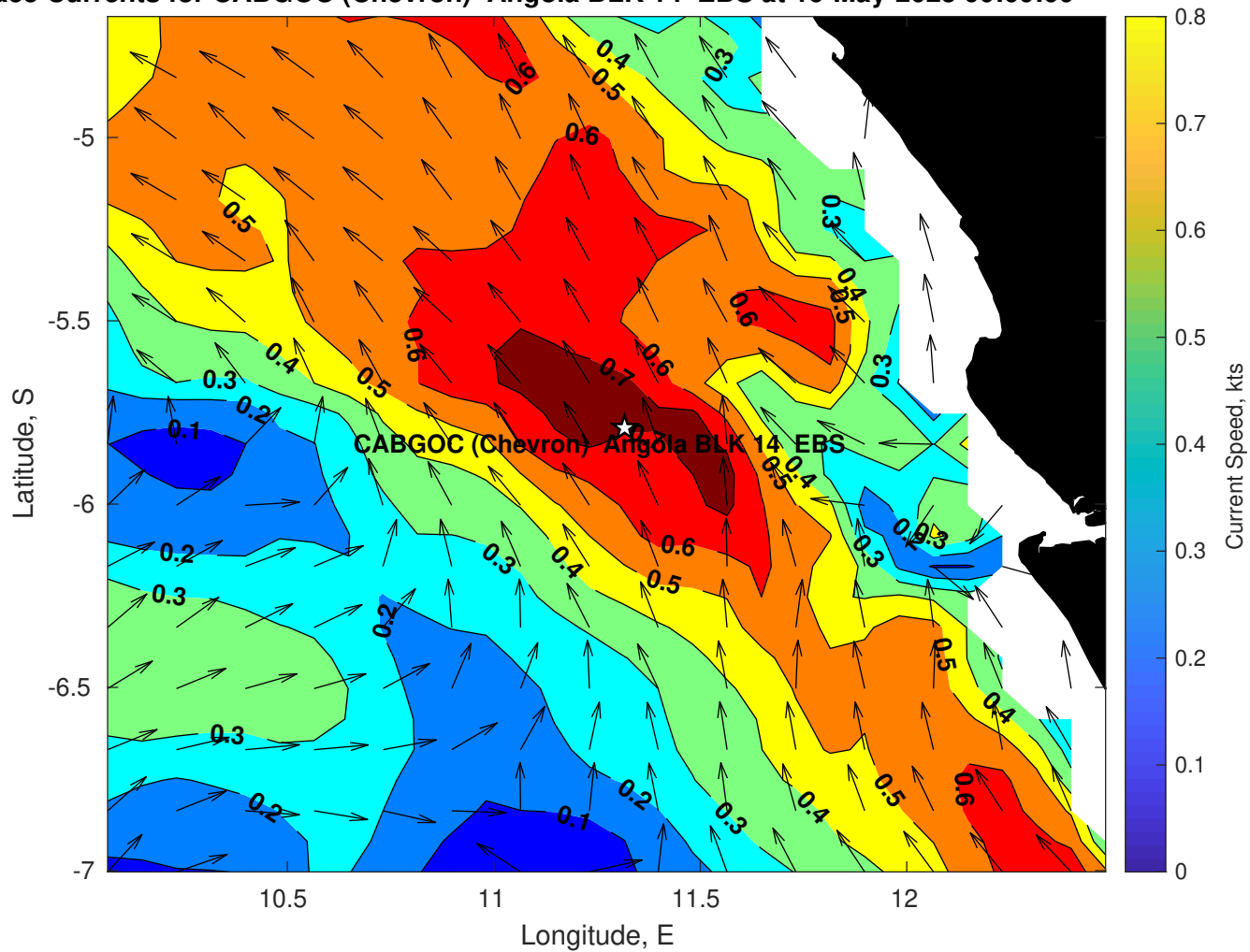
Surface Currents for CABGOC (Chevron) Angola BLK 14 EBS at 16-May-2025 00:00:00
