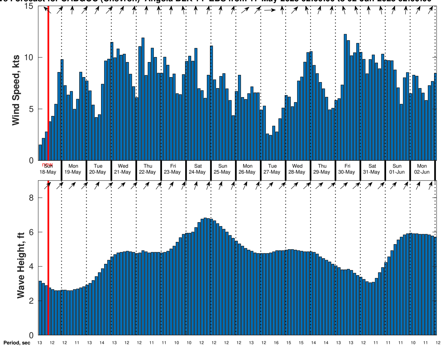
Wind & Wave Forecast for CABGOC (Chevron) Angola BLK 14 EBS from 17-May-2025 02:00:00 to 02-Jun-2025 02:00:00
