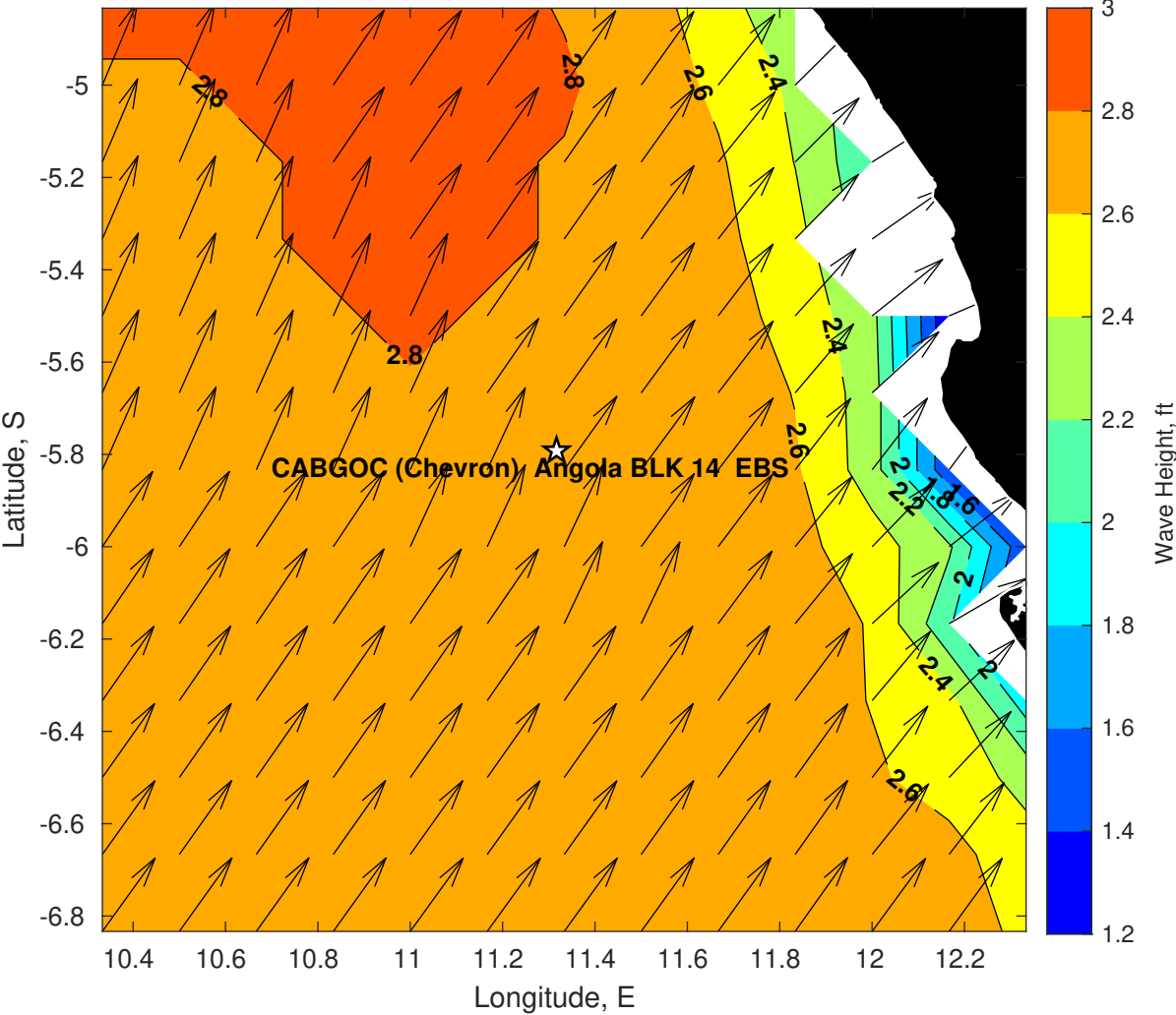
Wave Height (ft) for CABGOC (Chevron) Angola BLK 14 EBS at 17-May-2025 09:00:00
