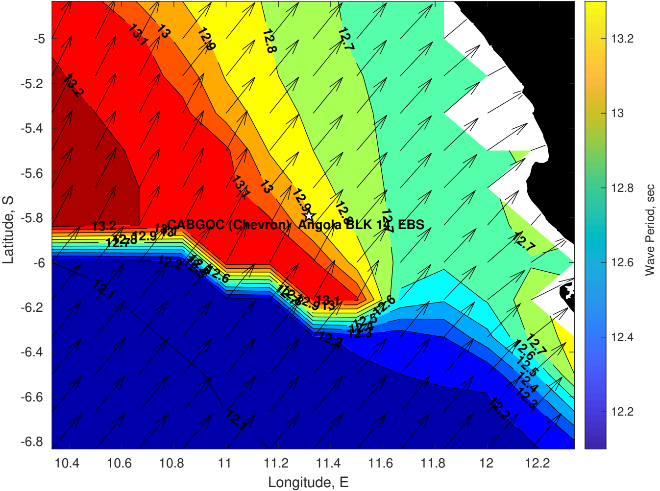
Wave Period (sec) for CABGOC (Chevron) Angola BLK 14 EBS at 17-May-2025 09:00:00
