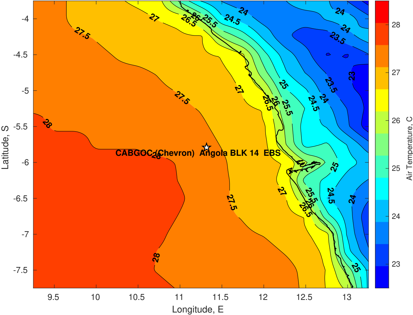
Air Temperature (C) for CABGOC (Chevron) Angola BLK 14 EBS at 17-May-2025
