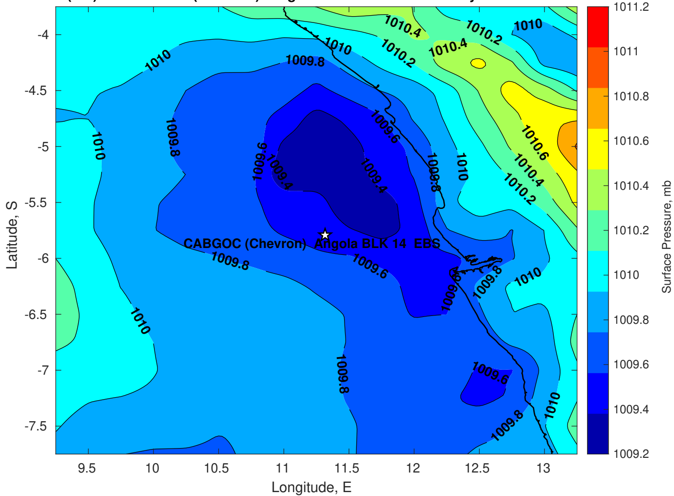
Surface Pressure (mb) for CABGOC (Chevron) Angola BLK 14 EBS at 17-May-2025 00:00:00
