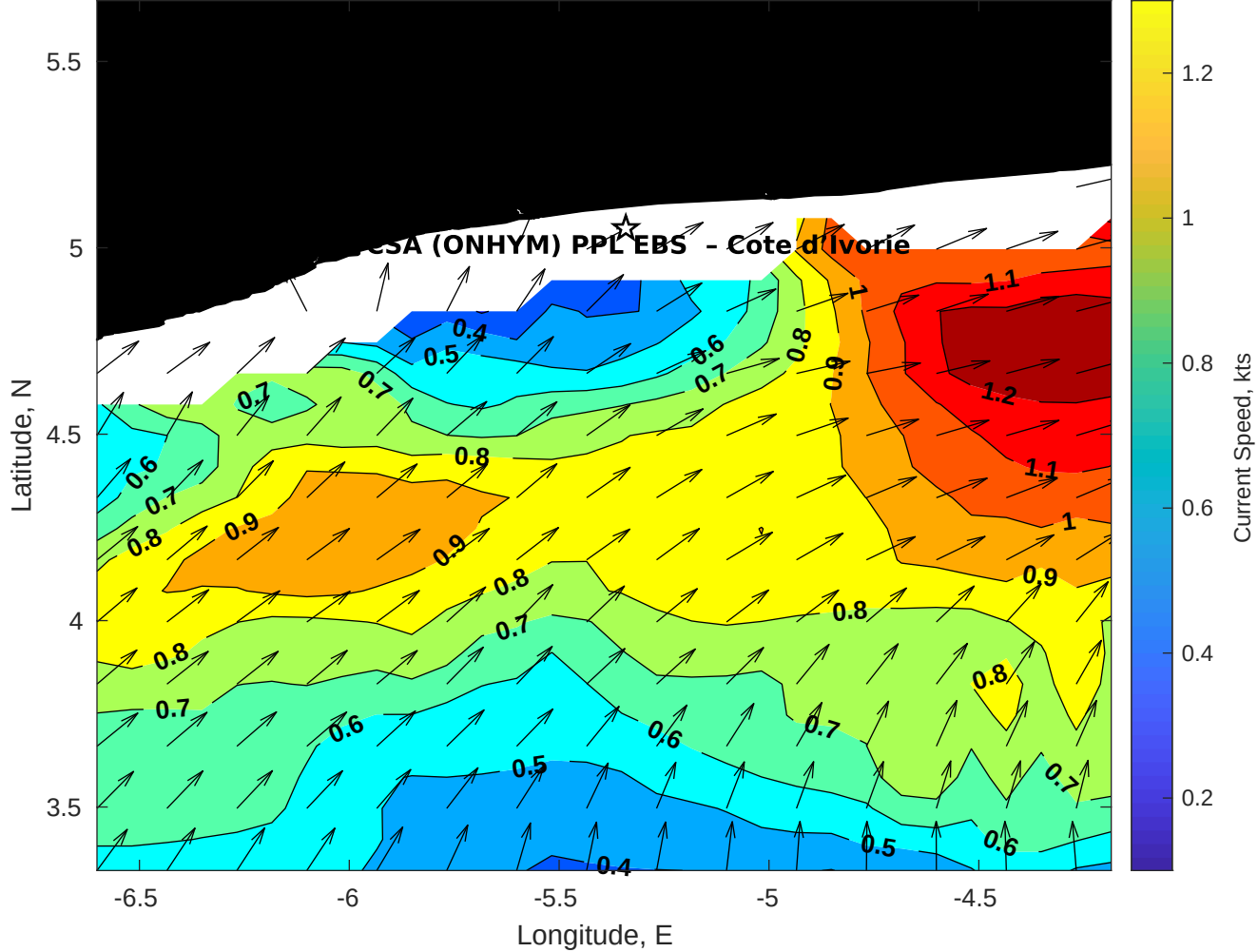
Surface Currents for CSA (ONHYM) PPL EBS - Cote d'Ivoire at 16-May-2025 00:00:00
