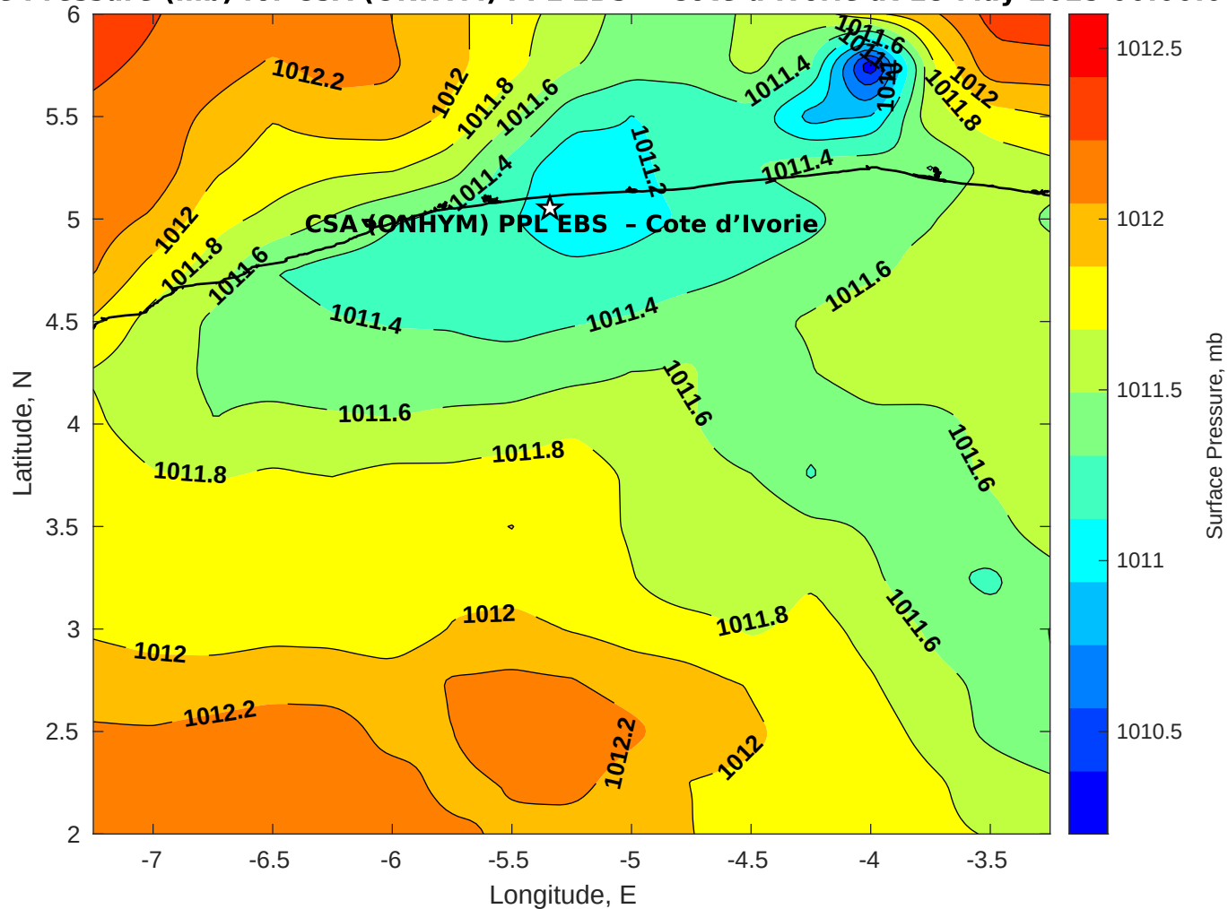
Surface Pressure (mb) for CSA (ONHYM) PPL EBS - Cote d'Ivoire at 18-May-2025 00:00:00
