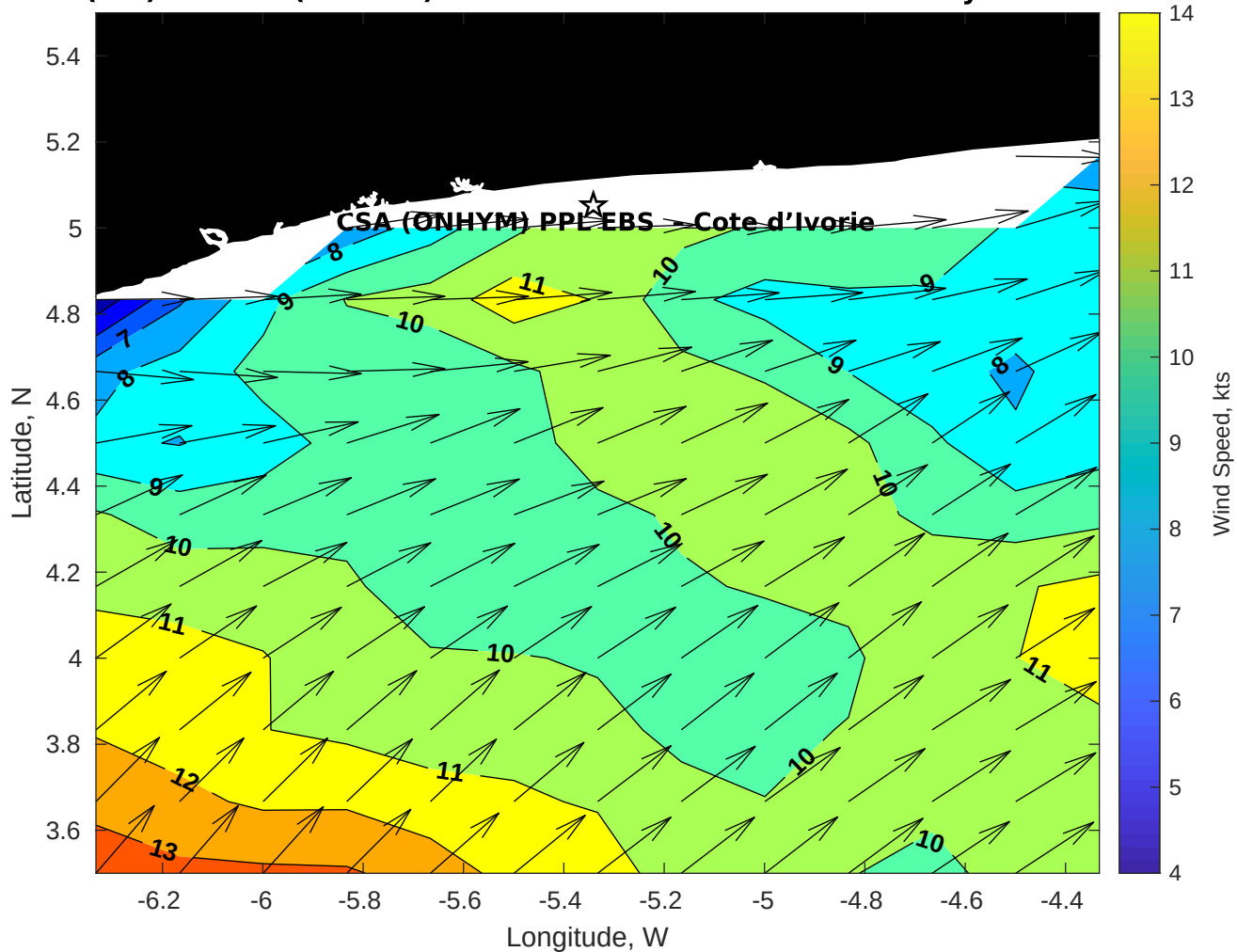
Winds (kts) for CSA (ONHYM) PPL EBS - Cote d'Ivoire at 17-May-2025 09:00:00
