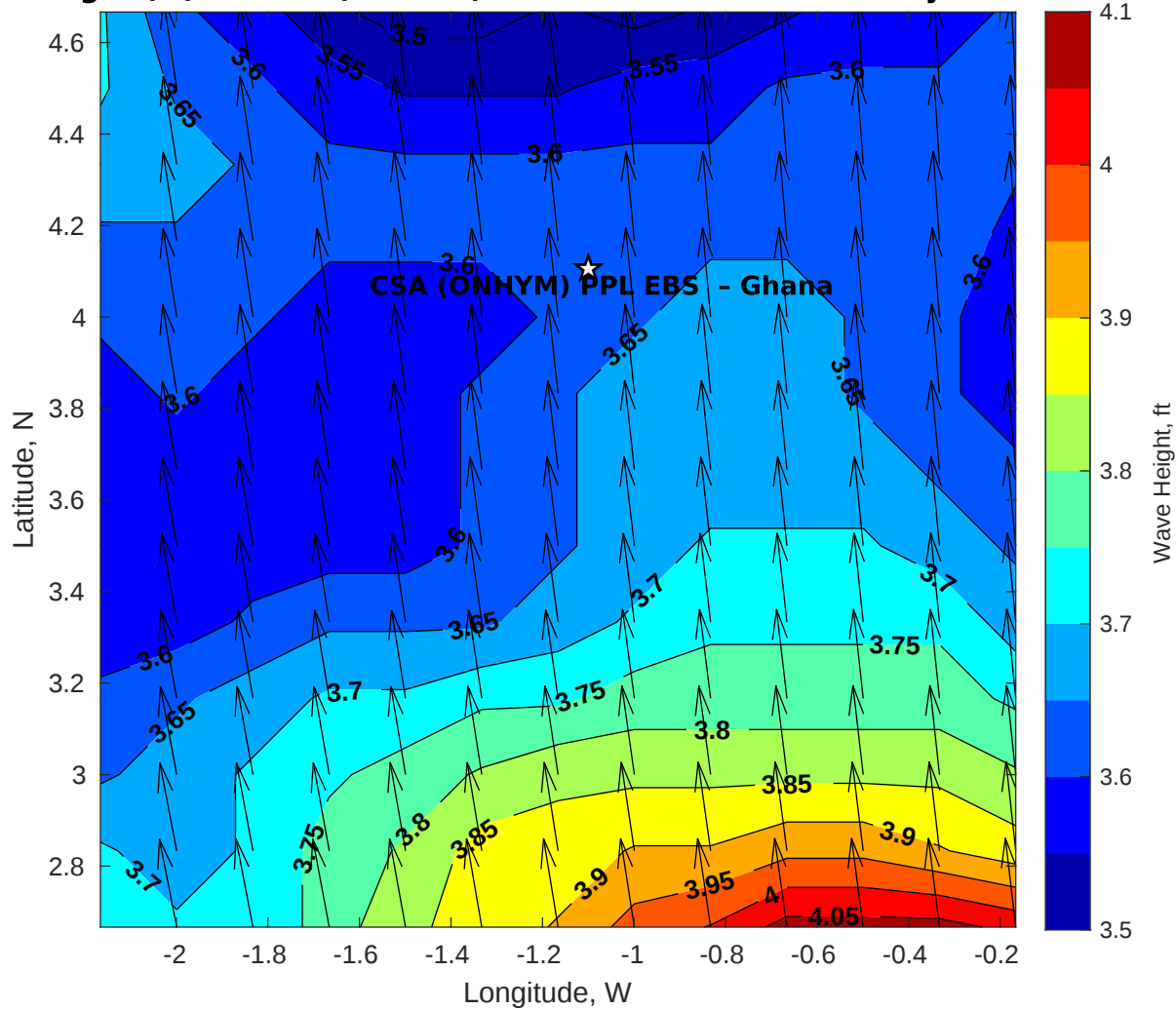
Wave Height (ft) for CSA (ONHYM) PPL EBS - Ghana at 17-May-2025 09:00:00
