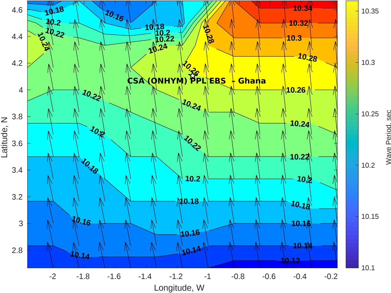
Wave Period (sec) for CSA (ONHYM) PPL EBS - Ghana at 17-May-2025 09:00:00
