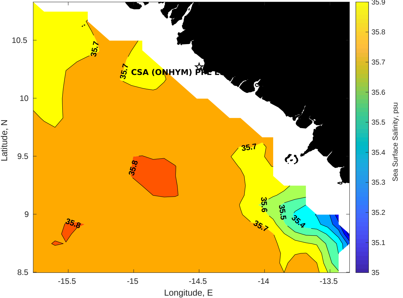
Surface Salinity for CSA (ONHYM) PPL EBS - Guinea at 16-May-2025 00:00:00
