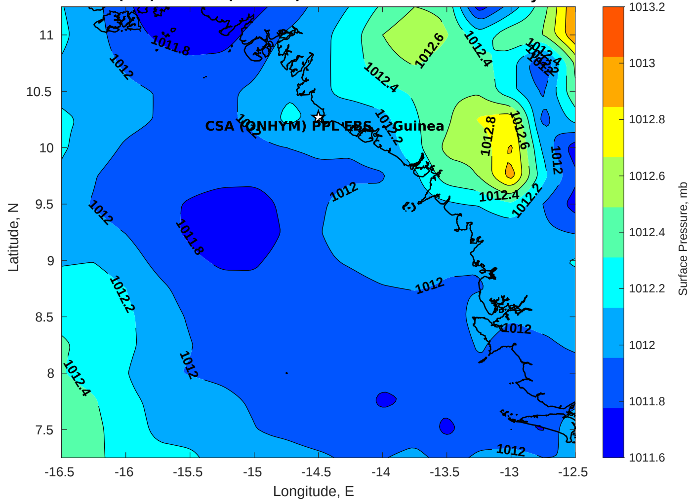
Surface Pressure (mb) for CSA (ONHYM) PPL EBS - Guinea at 18-May-2025 00:00:00
