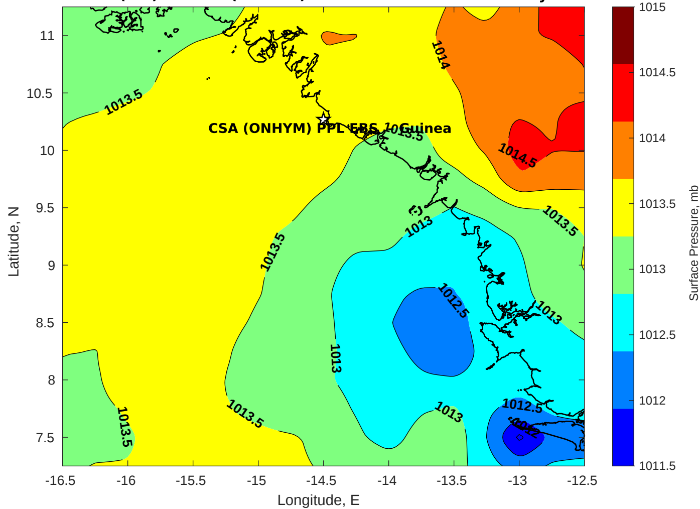
Surface Pressure (mb) for CSA (ONHYM) PPL EBS - Guinea at 19-May-2025 00:00:00
