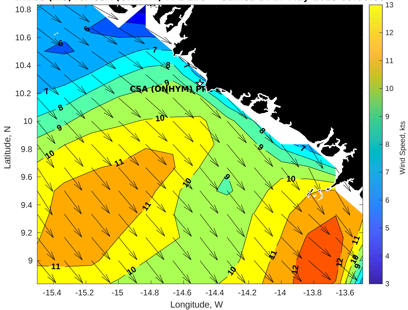
Winds (kts) for CSA (ONHYM) PPL EBS - Guinea at 17-May-2025 09:00:00
