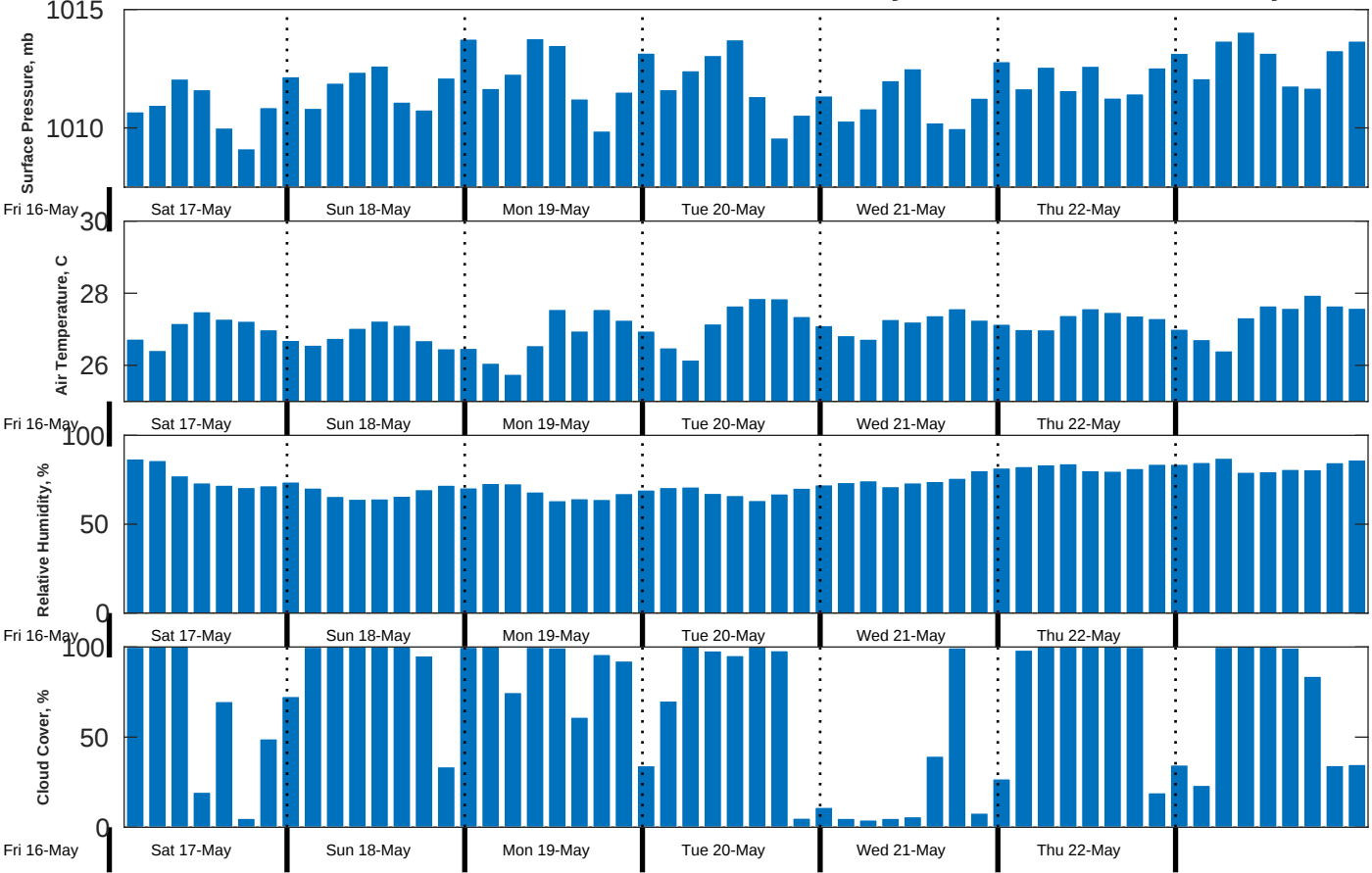
Met Forecast for CSA (ONHYM) PPL EBS - Guinea from 17-May-2025 00:00:00 to 24-May-2025 00:00:00
