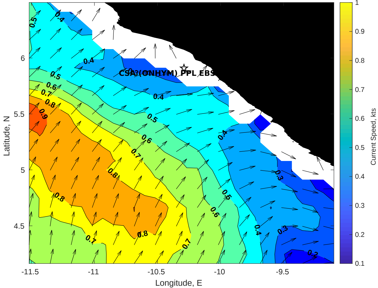
Surface Currents for CSA (ONHYM) PPL EBS - Liberia at 16-May-2025 00:00:00
