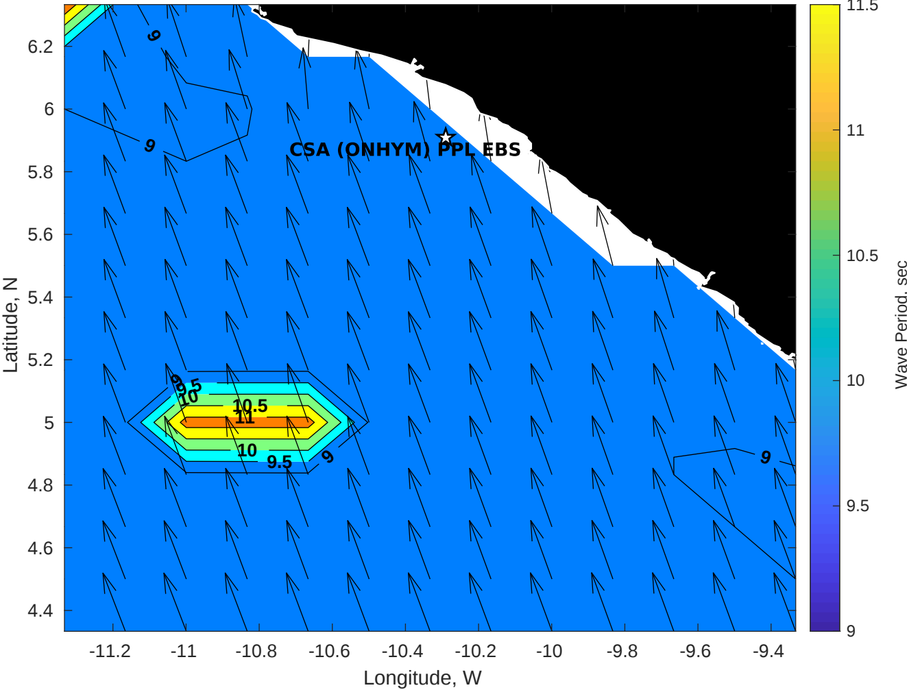
Wave Period (sec) for CSA (ONHYM) PPL EBS - Liberia at 17-May-2025 09:00:00
