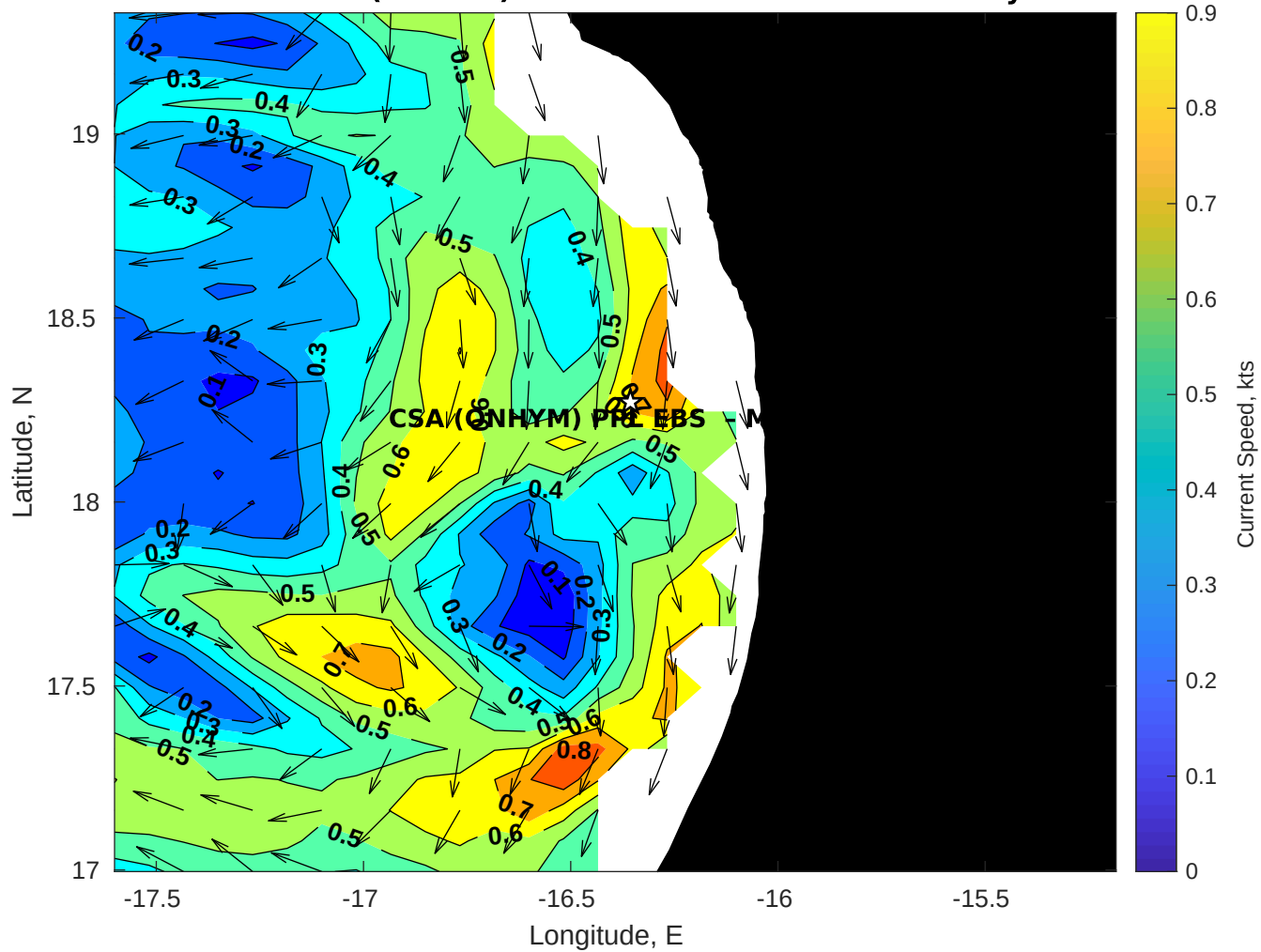
Surface Currents for CSA (ONHYM) PPL EBS - Mauritania at 16-May-2025 00:00:00
