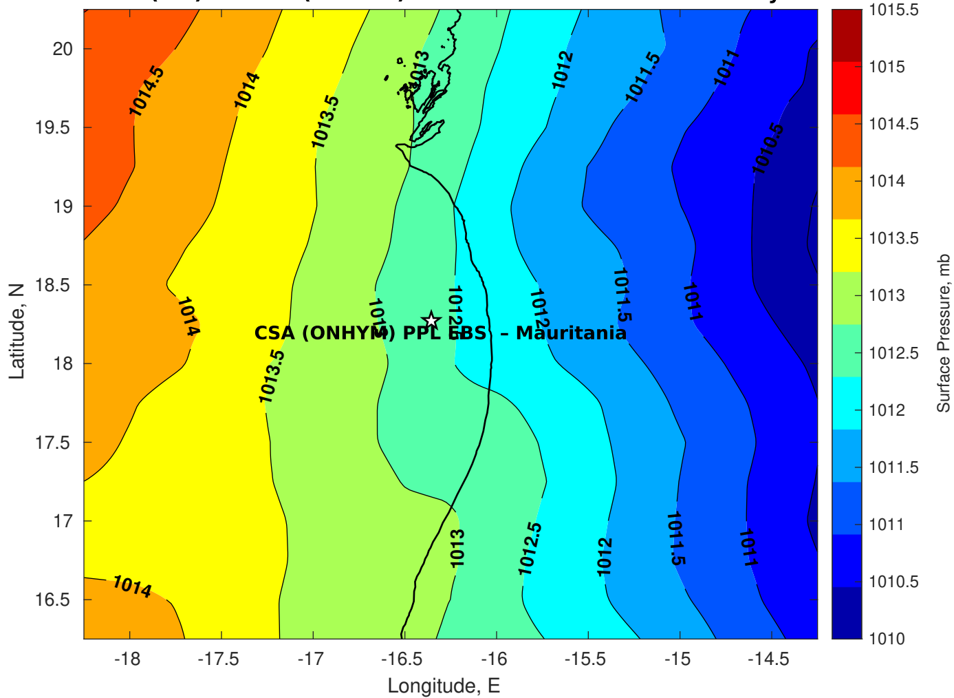
Surface Pressure (mb) for CSA (ONHYM) PPL EBS - Mauritania at 19-May-2025 00:00:00
