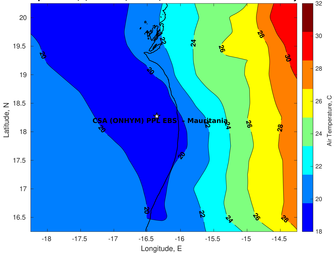
Air Temperature (C) for CSA (ONHYM) PPL EBS - Mauritania at 17-May-2025
