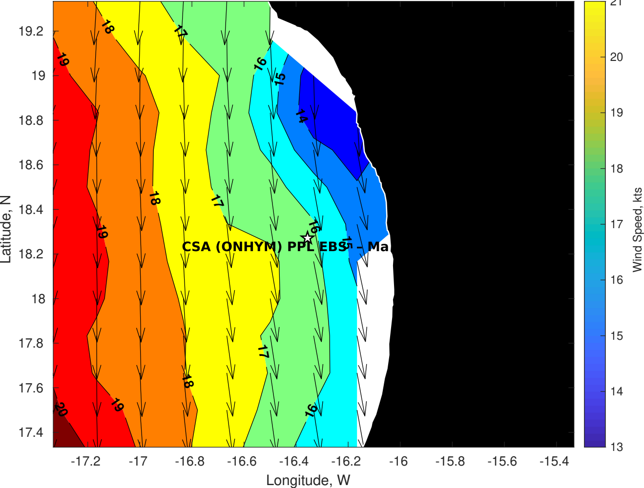
Winds (kts) for CSA (ONHYM) PPL EBS - Mauritania at 17-May-2025 09:00:00
