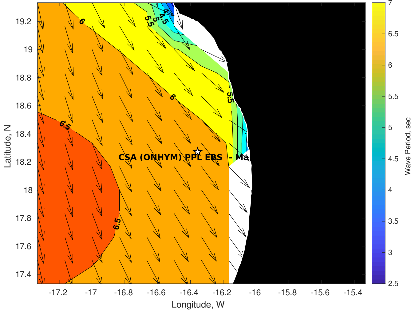
Wave Period (sec) for CSA (ONHYM) PPL EBS - Mauritania at 17-May-2025 09:00:00
