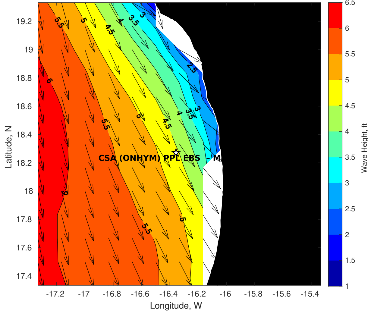
Wave Height (ft) for CSA (ONHYM) PPL EBS - Mauritania at 17-May-2025 09:00:00
