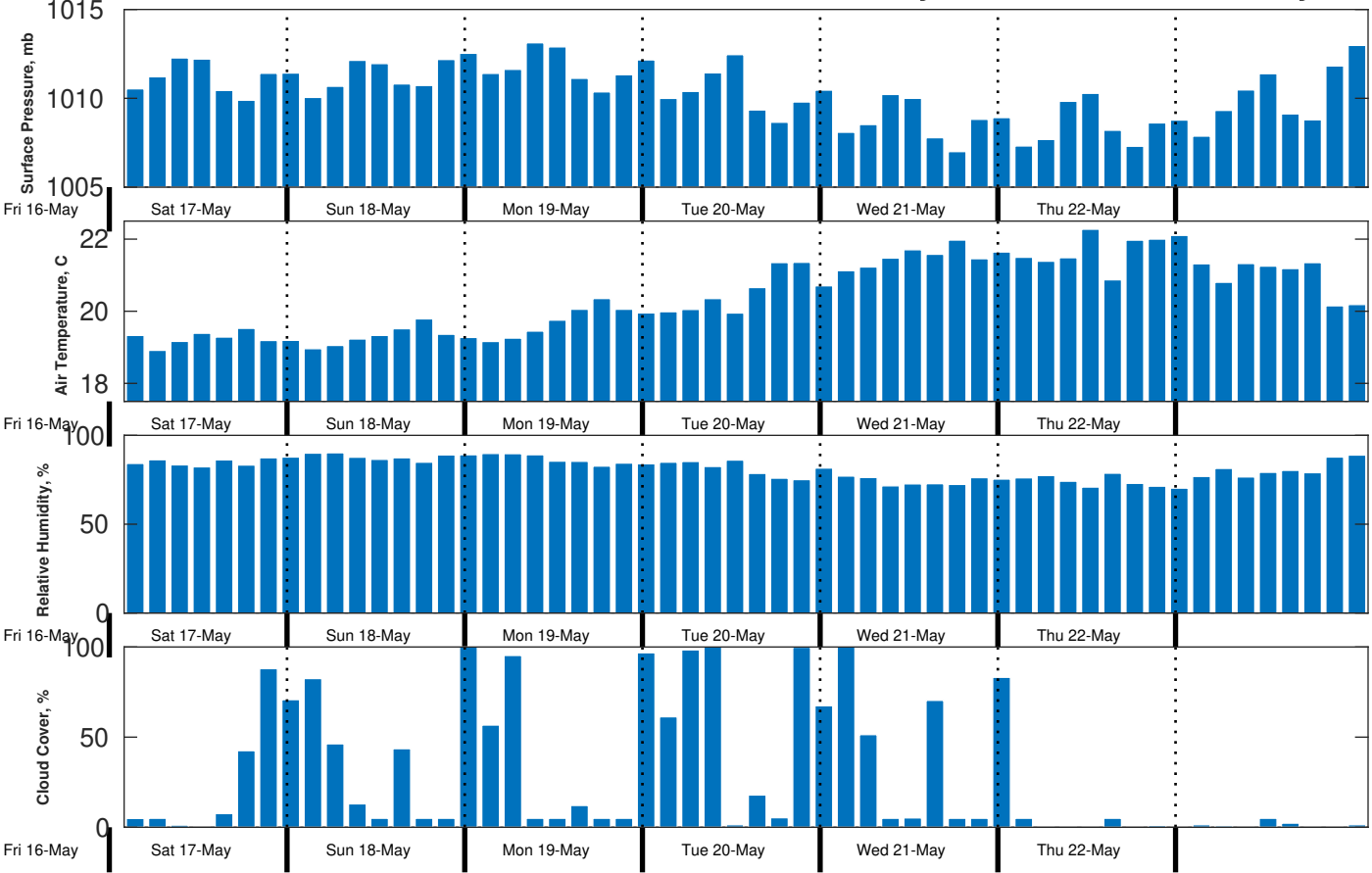
Met Forecast for CSA (ONHYM) PPL EBS - Mauritania from 17-May-2025 00:00:00 to 24-May-2025 00:00:00
