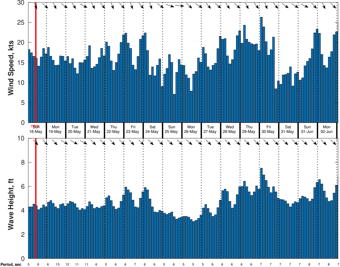
Wind & Wave Forecast for CSA (ONHYM) PPL EBS - Mauritania from 17-May-2025 01:00:00 to 02-Jun-2025 01:00:00
