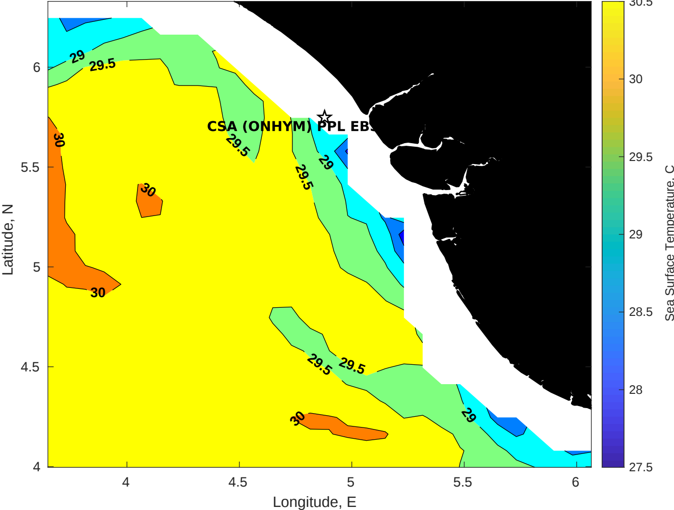
SST for CSA (ONHYM) PPL EBS - Nigeria at 16-May-2025 00:00:00
