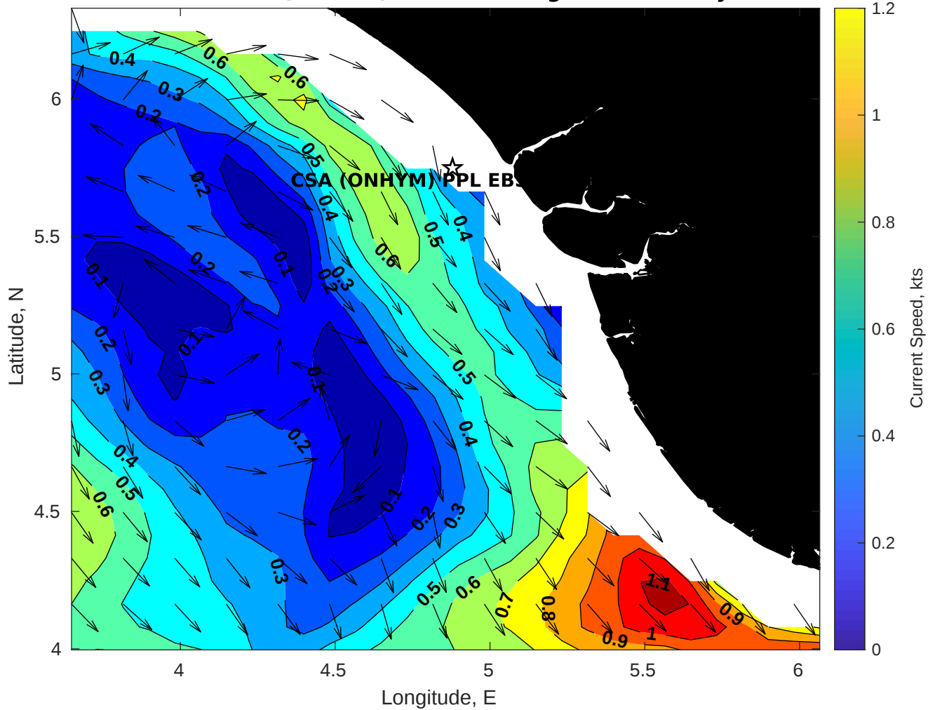
Surface Currents for CSA (ONHYM) PPL EBS - Nigeria at 16-May-2025 00:00:00
