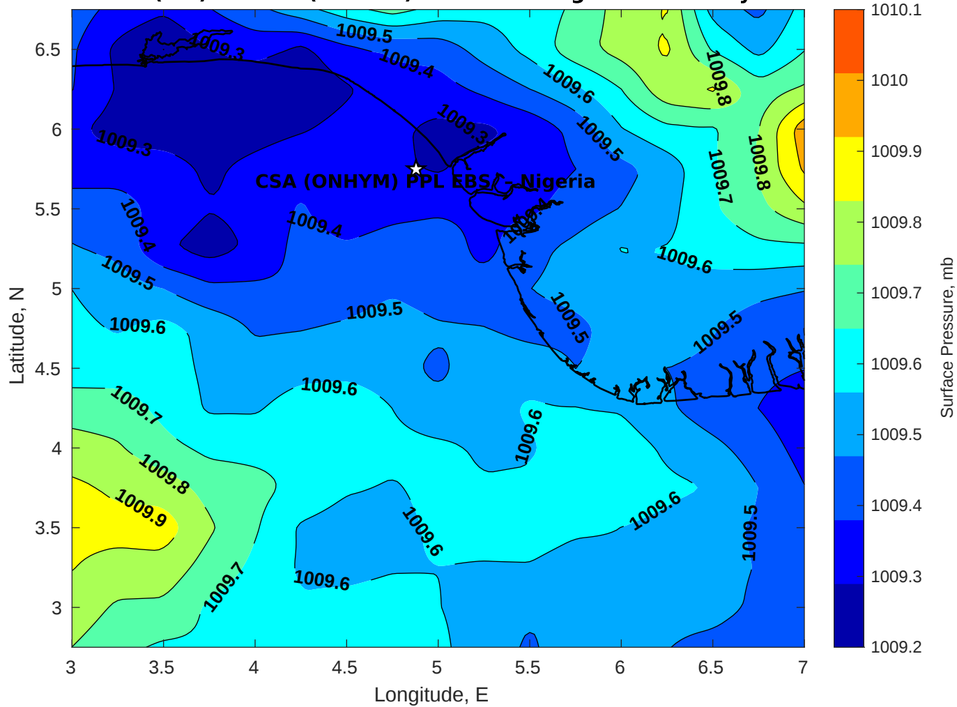
Surface Pressure (mb) for CSA (ONHYM) PPL EBS - Nigeria at 17-May-2025 00:00:00
