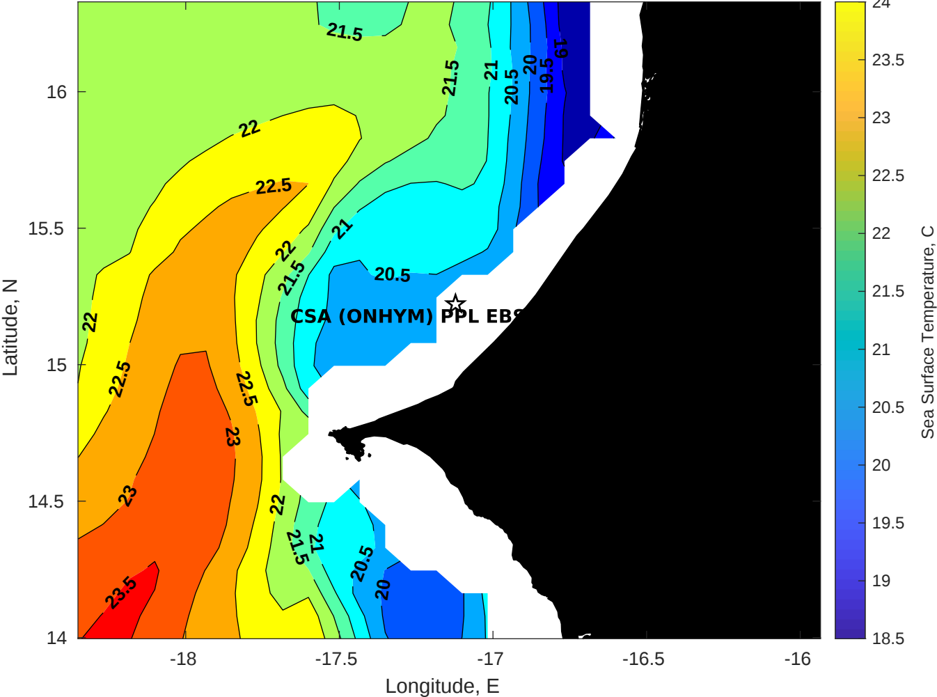
SST for CSA (ONHYM) PPL EBS - Senegal at 16-May-2025 00:00:00
