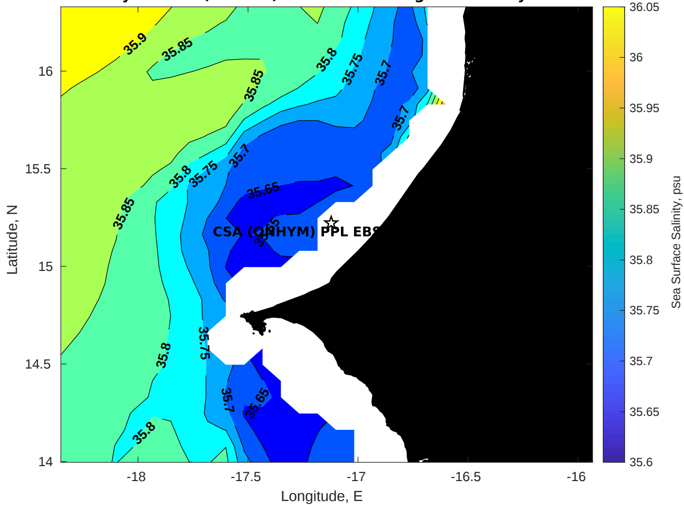
Surface Salinity for CSA (ONHYM) PPL EBS - Senegal at 16-May-2025 00:00:00
