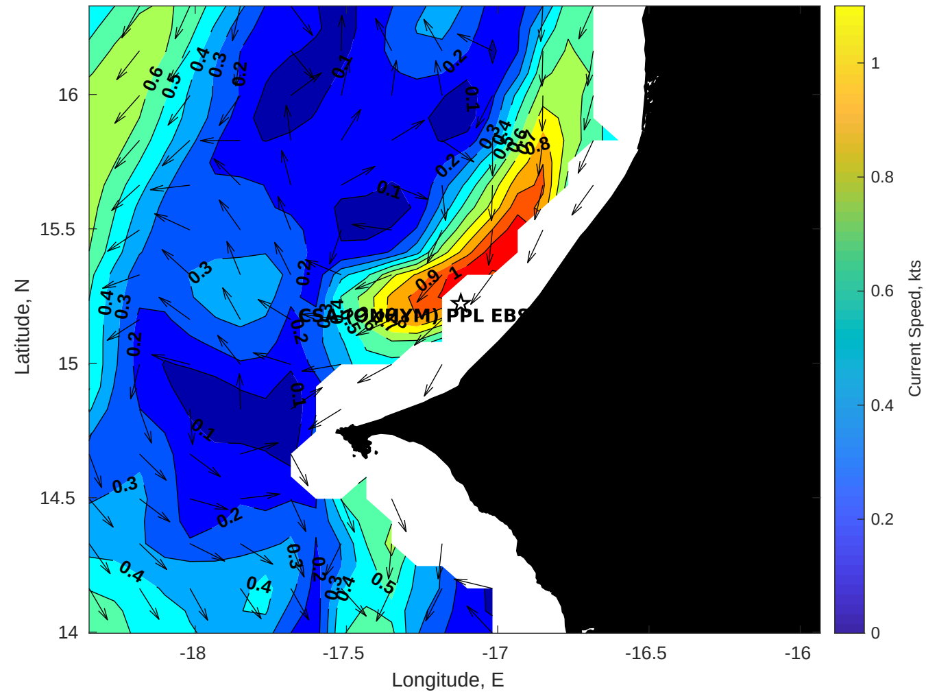
Surface Currents for CSA (ONHYM) PPL EBS - Senegal at 16-May-2025 00:00:00
