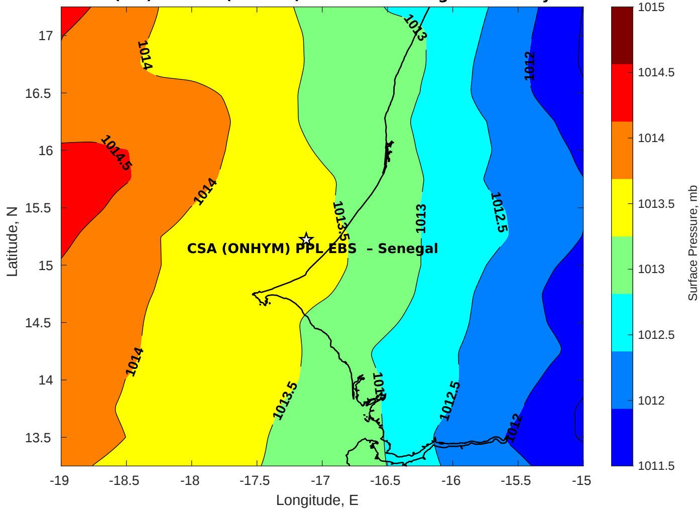
Surface Pressure (mb) for CSA (ONHYM) PPL EBS - Senegal at 19-May-2025 00:00:00
