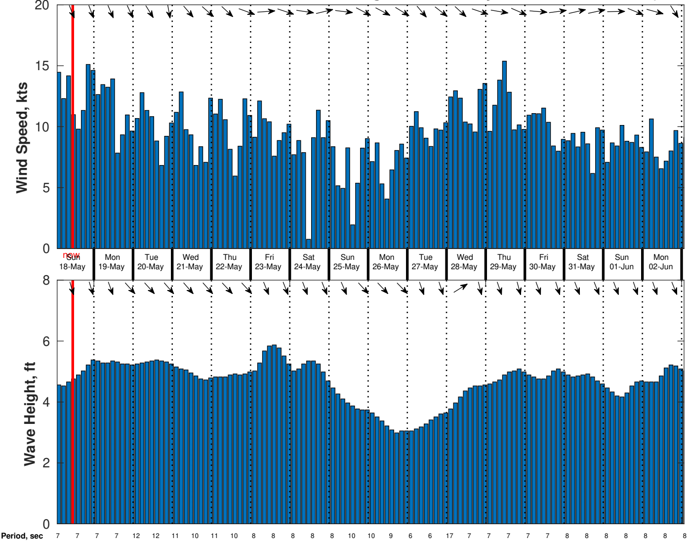
Wind & Wave Forecast for CSA (ONHYM) PPL EBS - Senegal from 17-May-2025 01:00:00 to 02-Jun-2025 01:00:00
