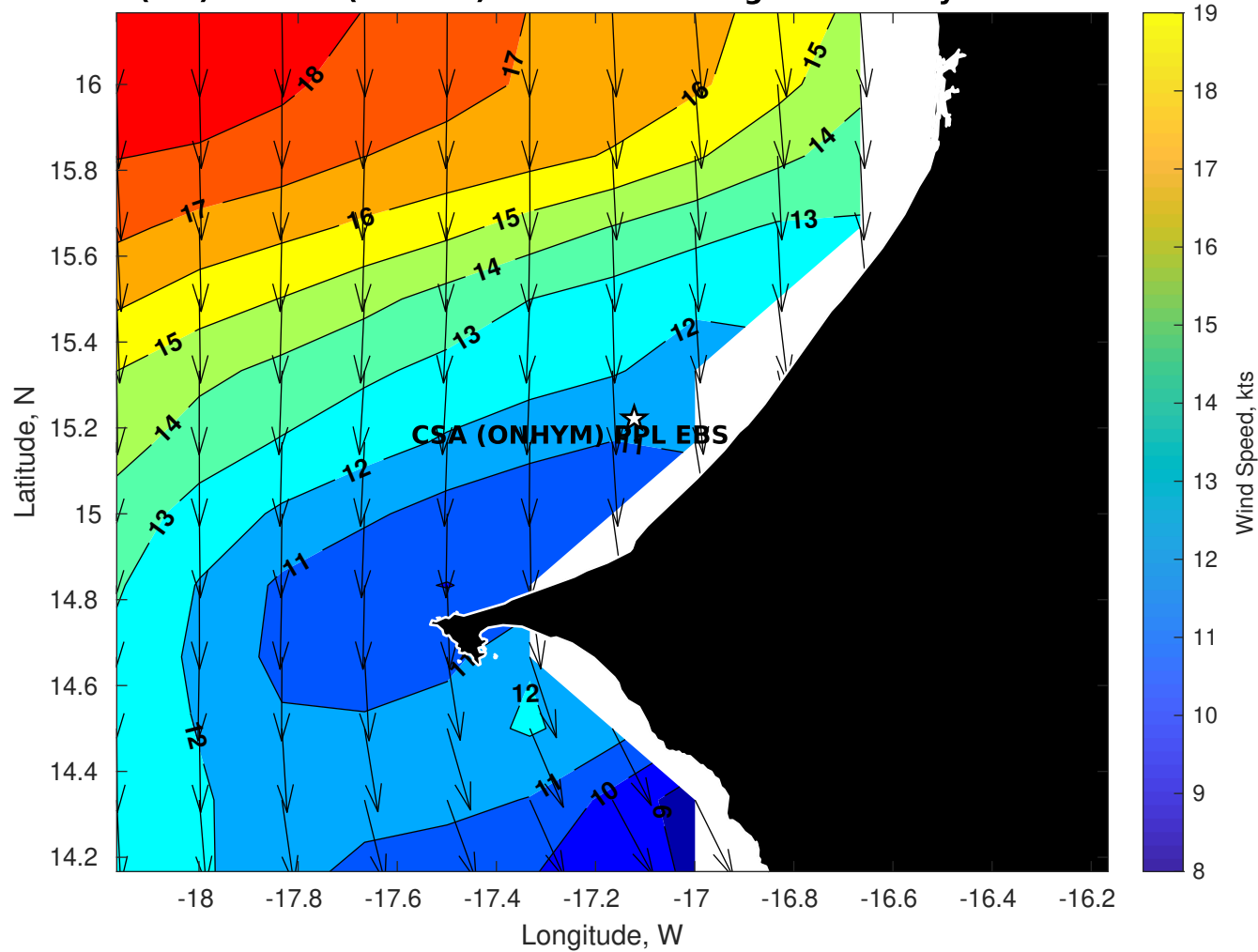
Winds (kts) for CSA (ONHYM) PPL EBS - Senegal at 17-May-2025 09:00:00
