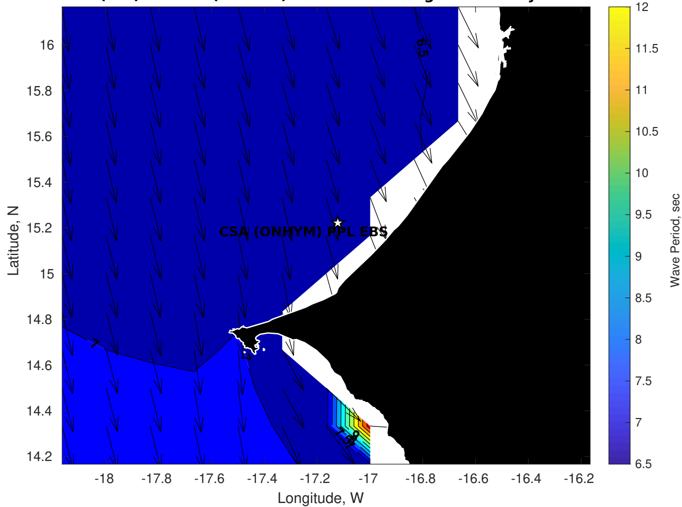
Wave Period (sec) for CSA (ONHYM) PPL EBS - Senegal at 17-May-2025 09:00:00
