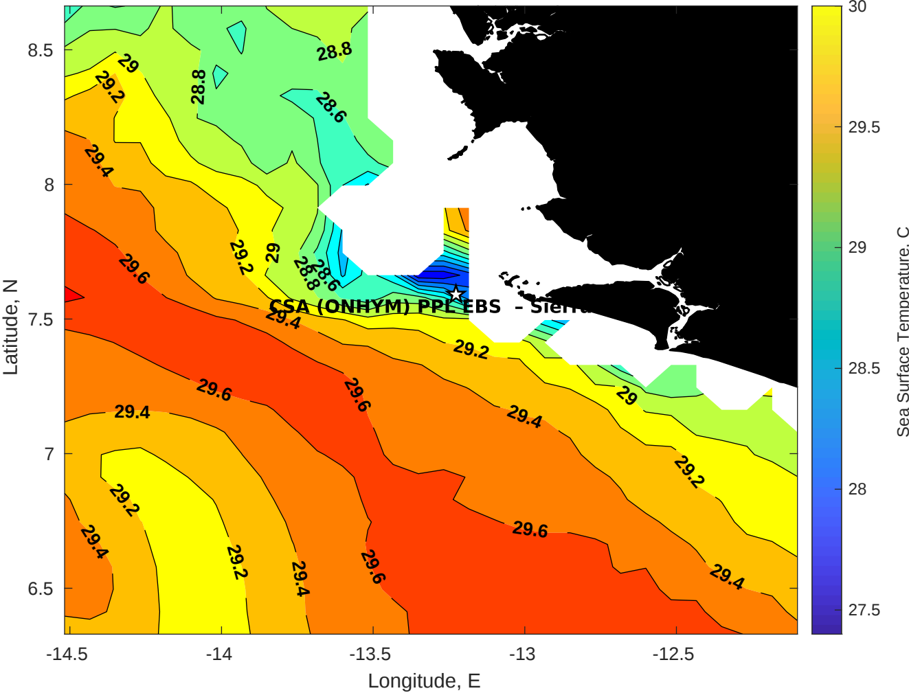
SST for CSA (ONHYM) PPL EBS - Sierra Leone at 16-May-2025 00:00:00
