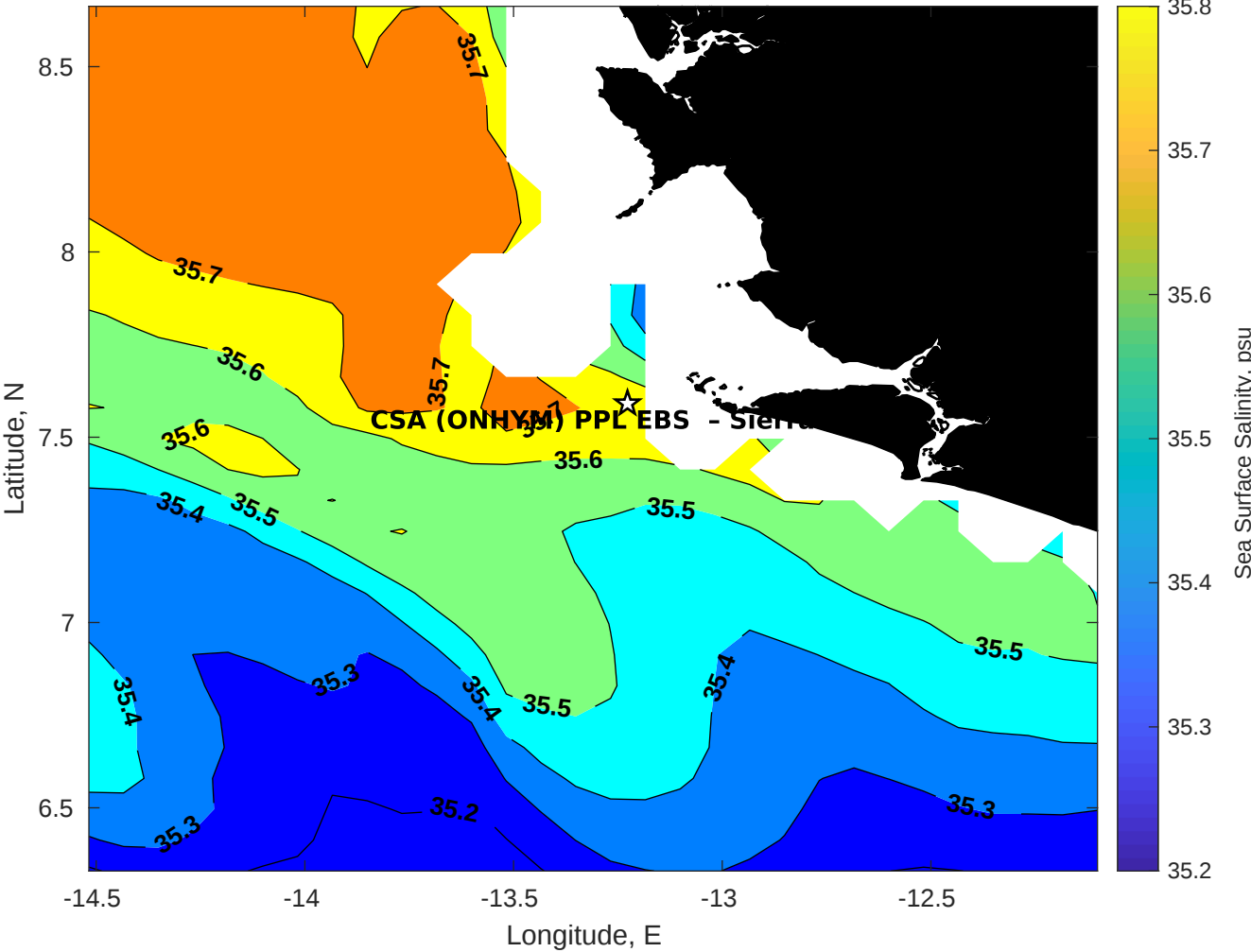
Surface Salinity for CSA (ONHYM) PPL EBS - Sierra Leone at 16-May-2025 00:00:00
