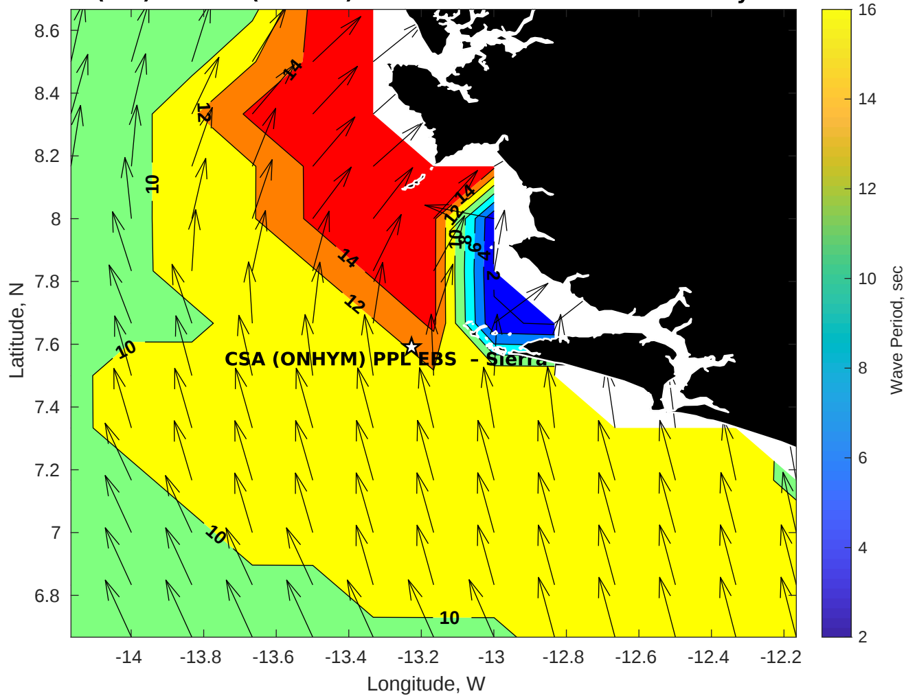
Wave Period (sec) for CSA (ONHYM) PPL EBS - Sierra Leone at 17-May-2025 09:00:00
