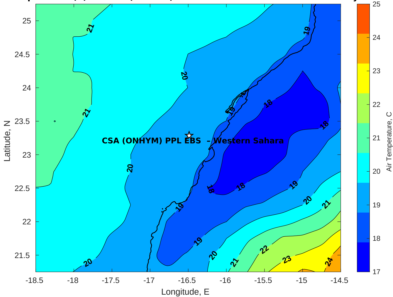
Air Temperature (C) for CSA (ONHYM) PPL EBS - Western Sahara at 17-May-2025
