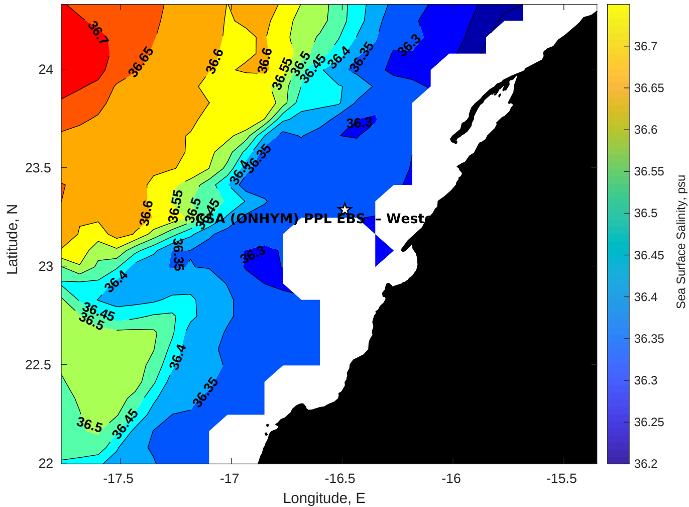
Surface Salinity for CSA (ONHYM) PPL EBS - Western Sahara at 16-May-2025 00:00:00
