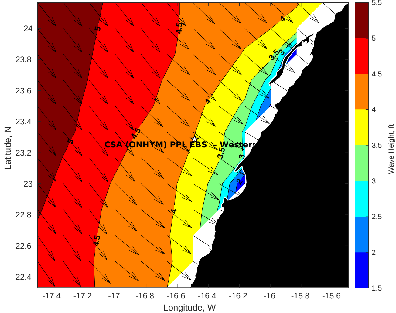
Wave Height (ft) for CSA (ONHYM) PPL EBS - Western Sahara at 17-May-2025 09:00:00
