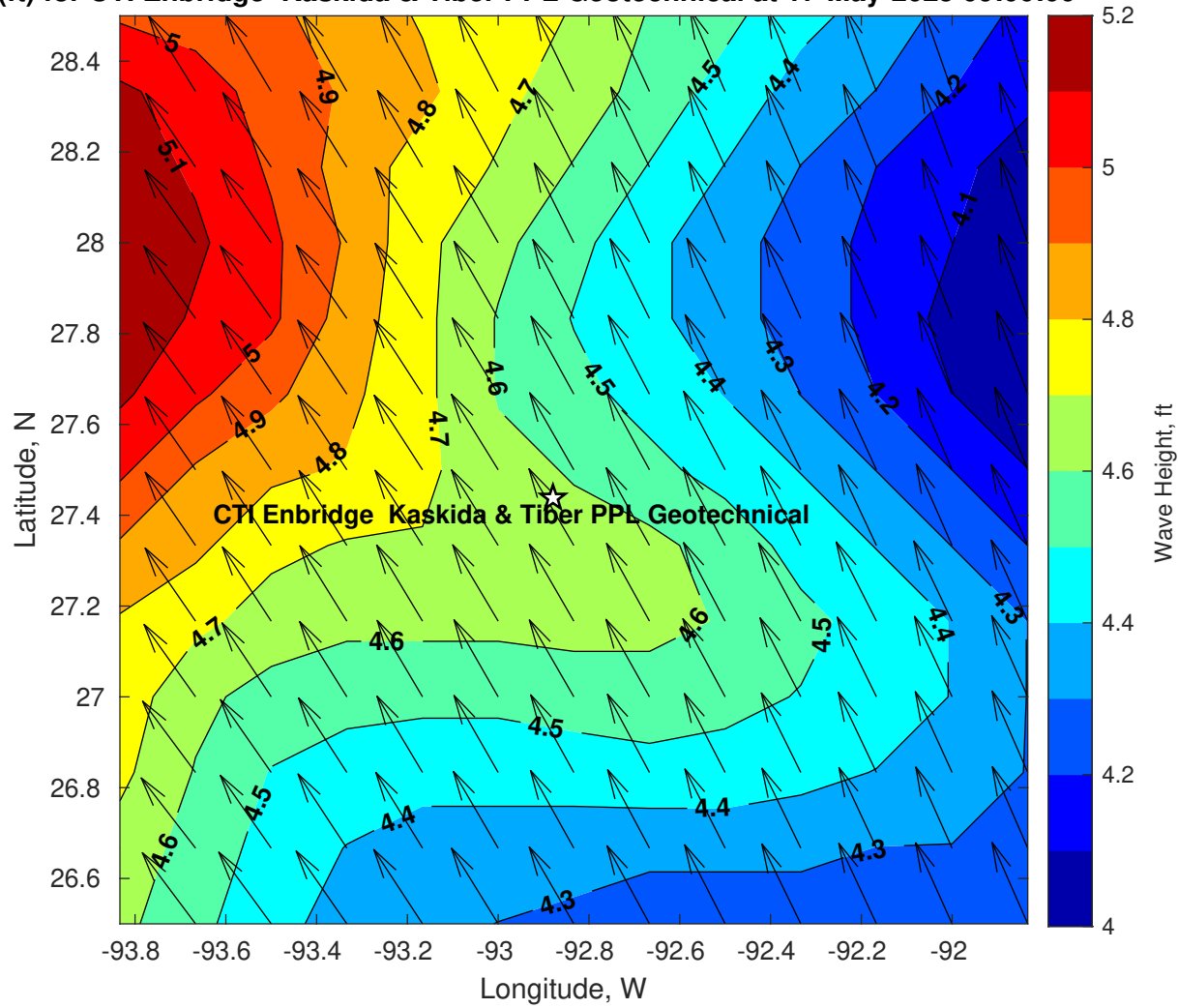
Wave Height (ft) for CTI Enbridge Kaskida & Tiber PPL Geotechnical at 17-May-2025 09:00:00
