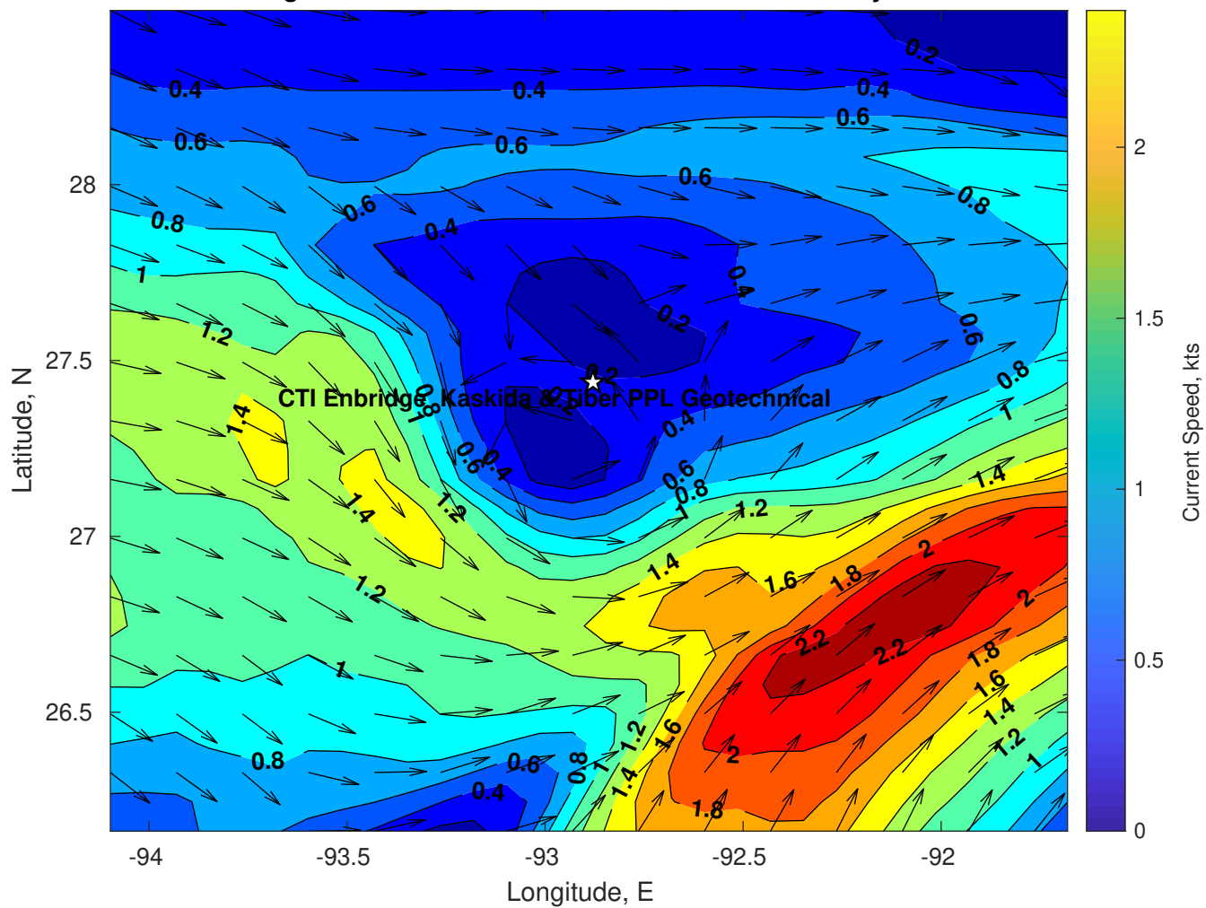
Surface Currents for CTI Enbridge Kaskida & Tiber PPL Geotechnical at 16-May-2025 00:00:00
