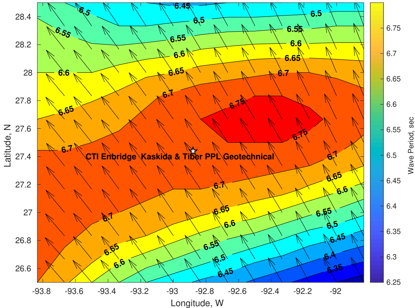
Wave Period (sec) for CTI Enbridge Kaskida & Tiber PPL Geotechnical at 17-May-2025 09:00:00
