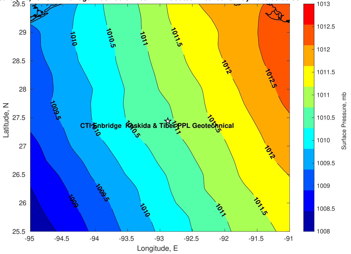
Surface Pressure (mb) for CTI Enbridge Kaskida & Tiber PPL Geotechnical at 19-May-2025 00:00:00
