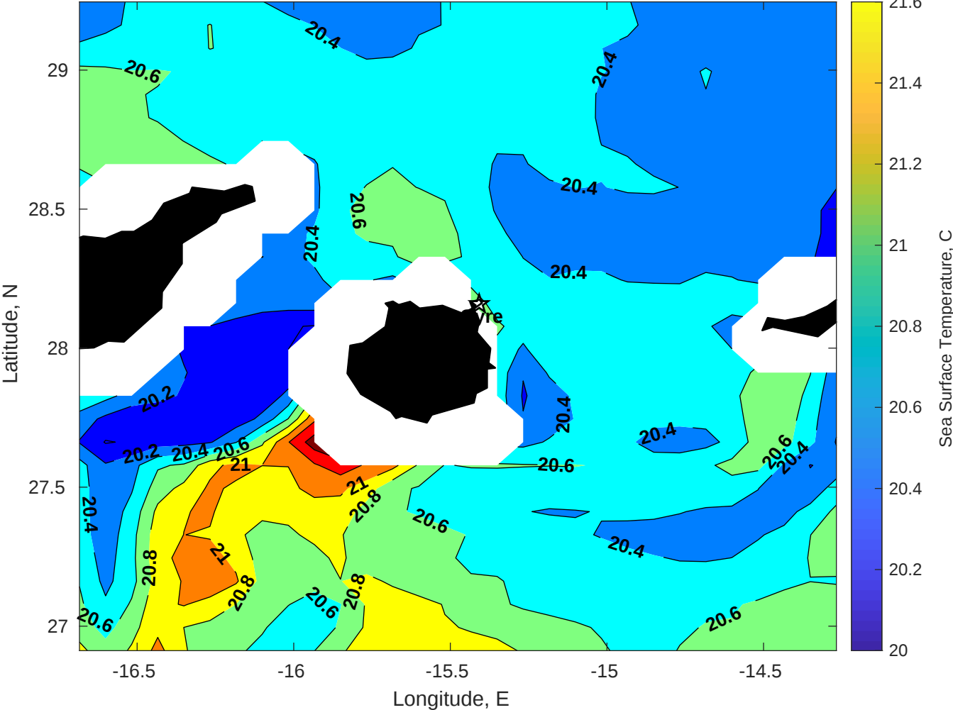
SST for Gyre at 16-May-2025 00:00:00
