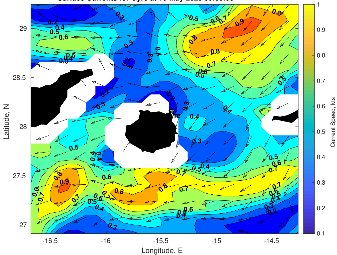
Surface Currents for Gyre at 16-May-2025 00:00:00
