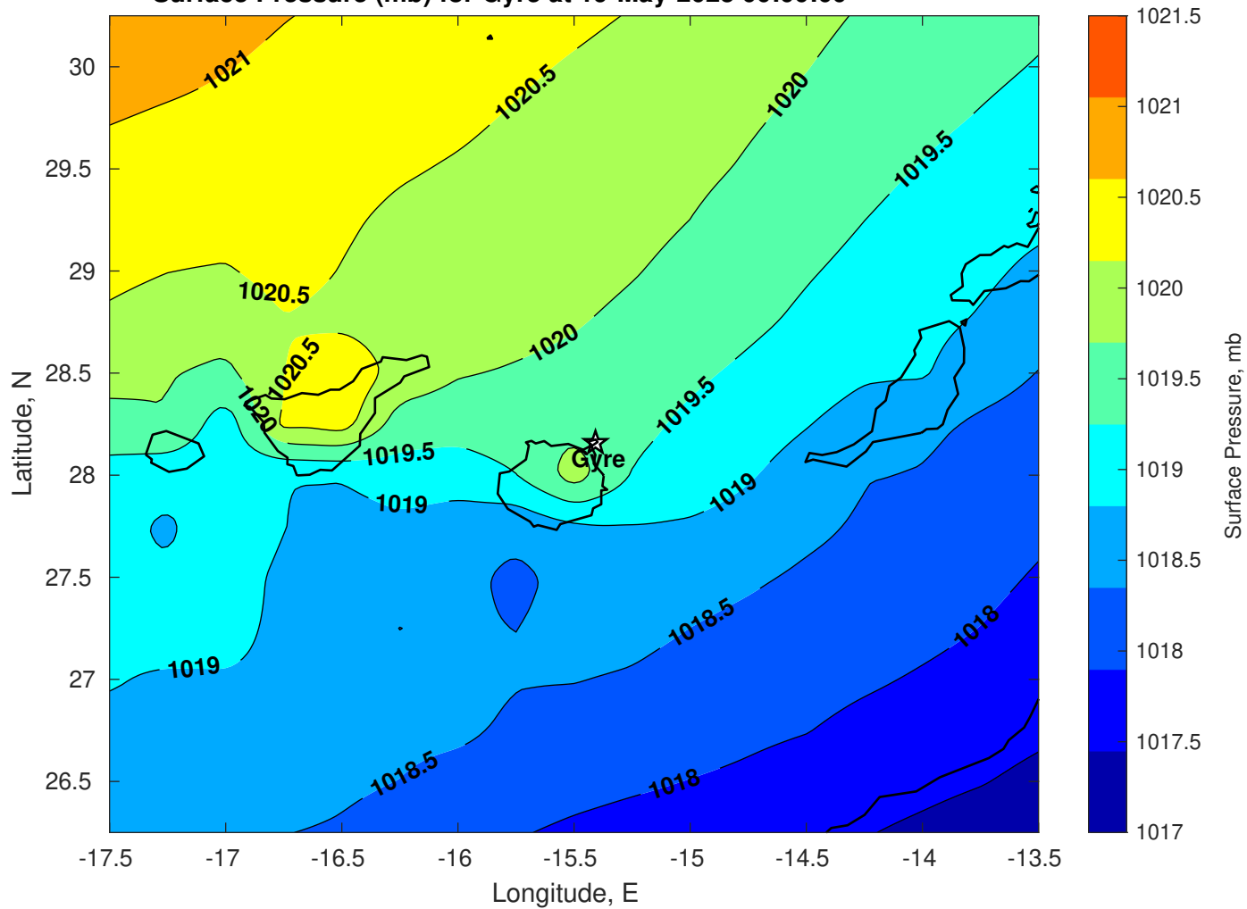
Surface Pressure (mb) for Gyre at 19-May-2025 00:00:00
