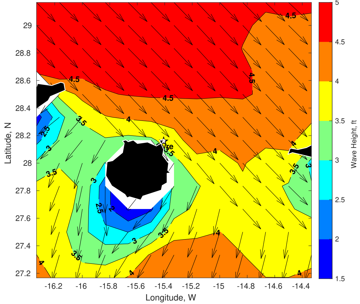
Wave Height (ft) for Gyre at 17-May-2025 09:00:00
