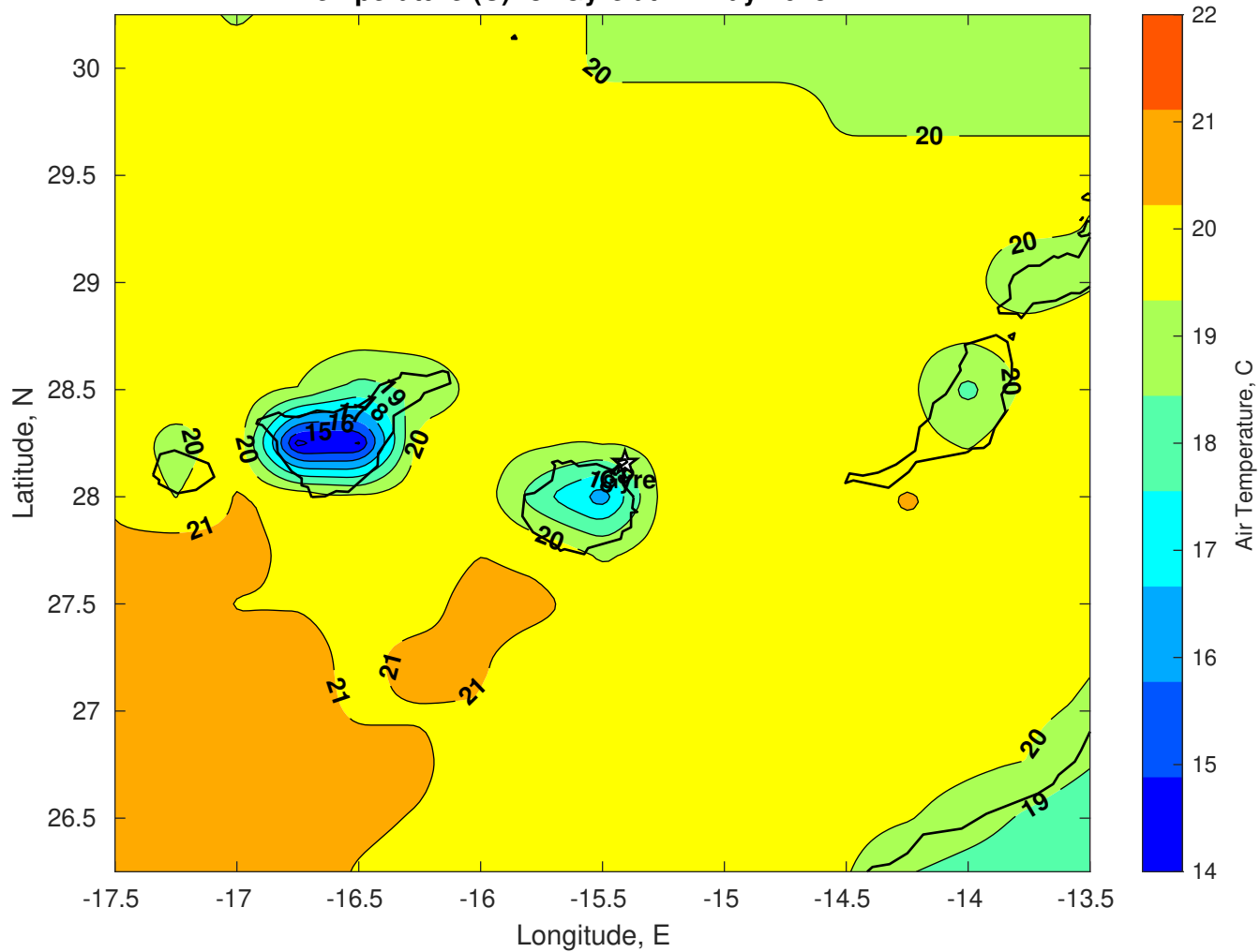
Air Temperature (C) for Gyre at 17-May-2025
