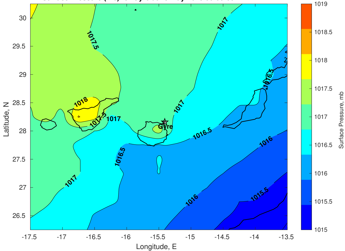
Surface Pressure (mb) for Gyre at 18-May-2025 00:00:00
