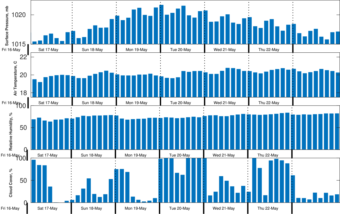
Met Forecast for Gyre from 16-May-2025 23:00:00 to 23-May-2025 23:00:00
