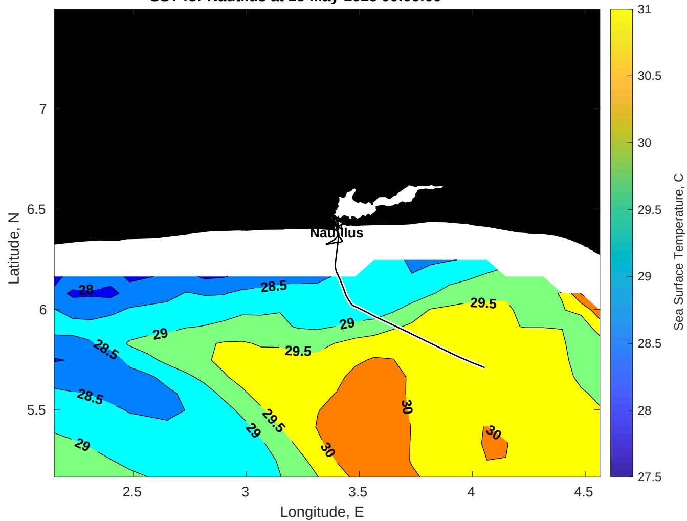
SST for Nautilus at 16-May-2025 00:00:00
