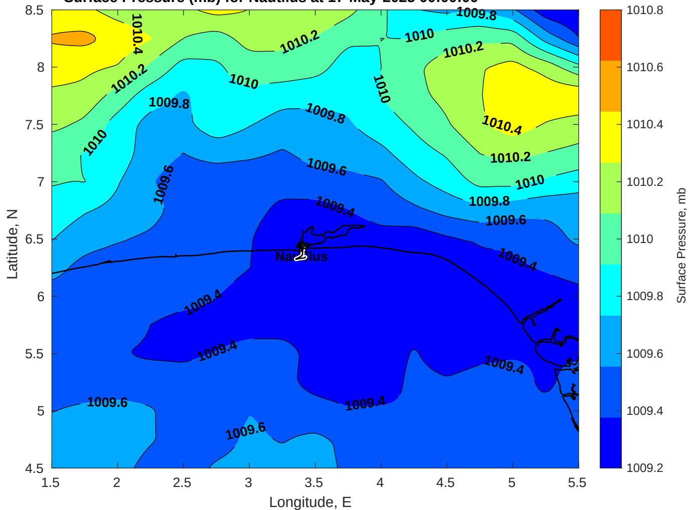
Surface Pressure (mb) for Nautilus at 17-May-2025 00:00:00
