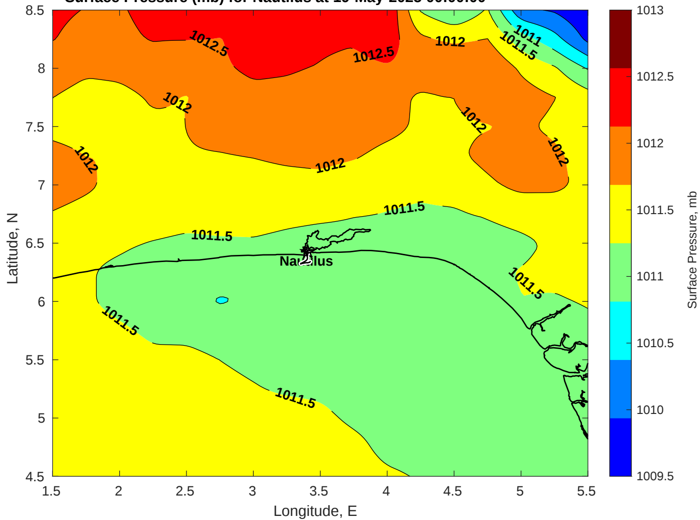
Surface Pressure (mb) for Nautilus at 19-May-2025 00:00:00
