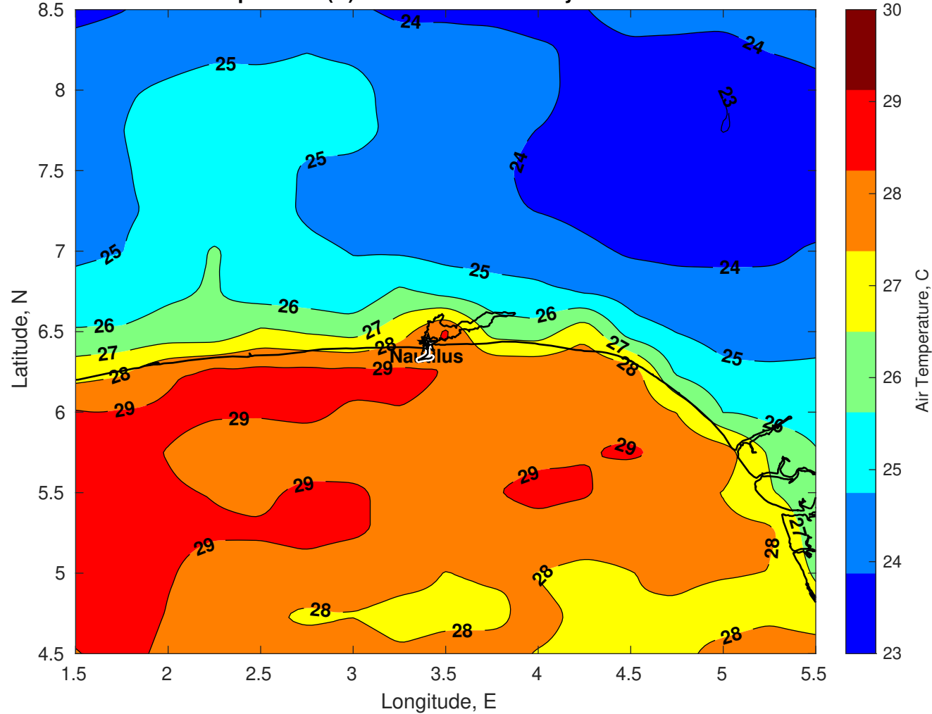
Air Temperature (C) for Nautilus at 17-May-2025
