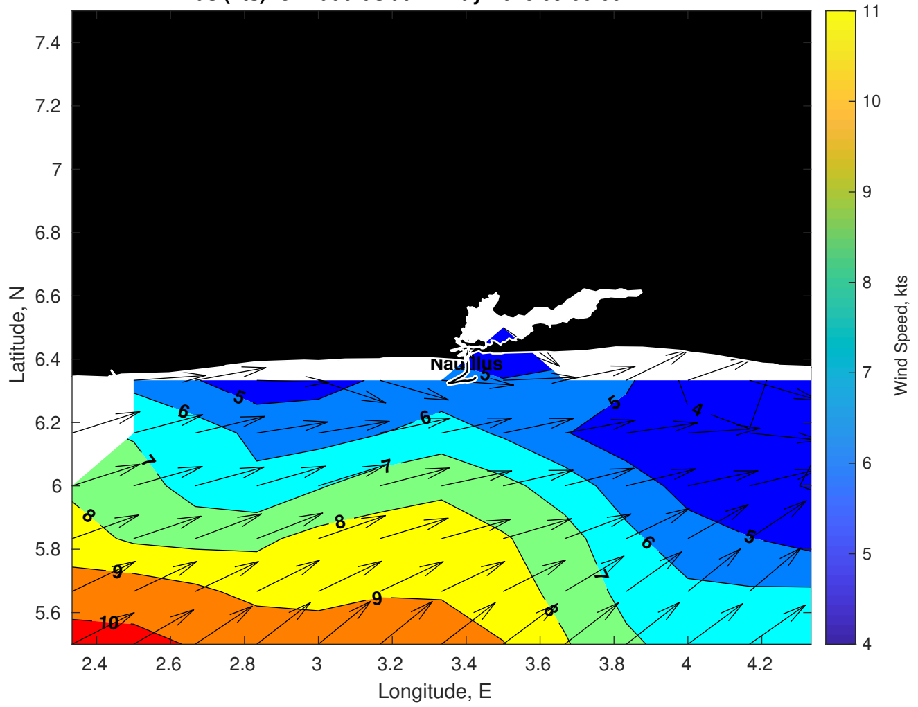
Winds (kts) for Nautilus at 17-May-2025 09:00:00
