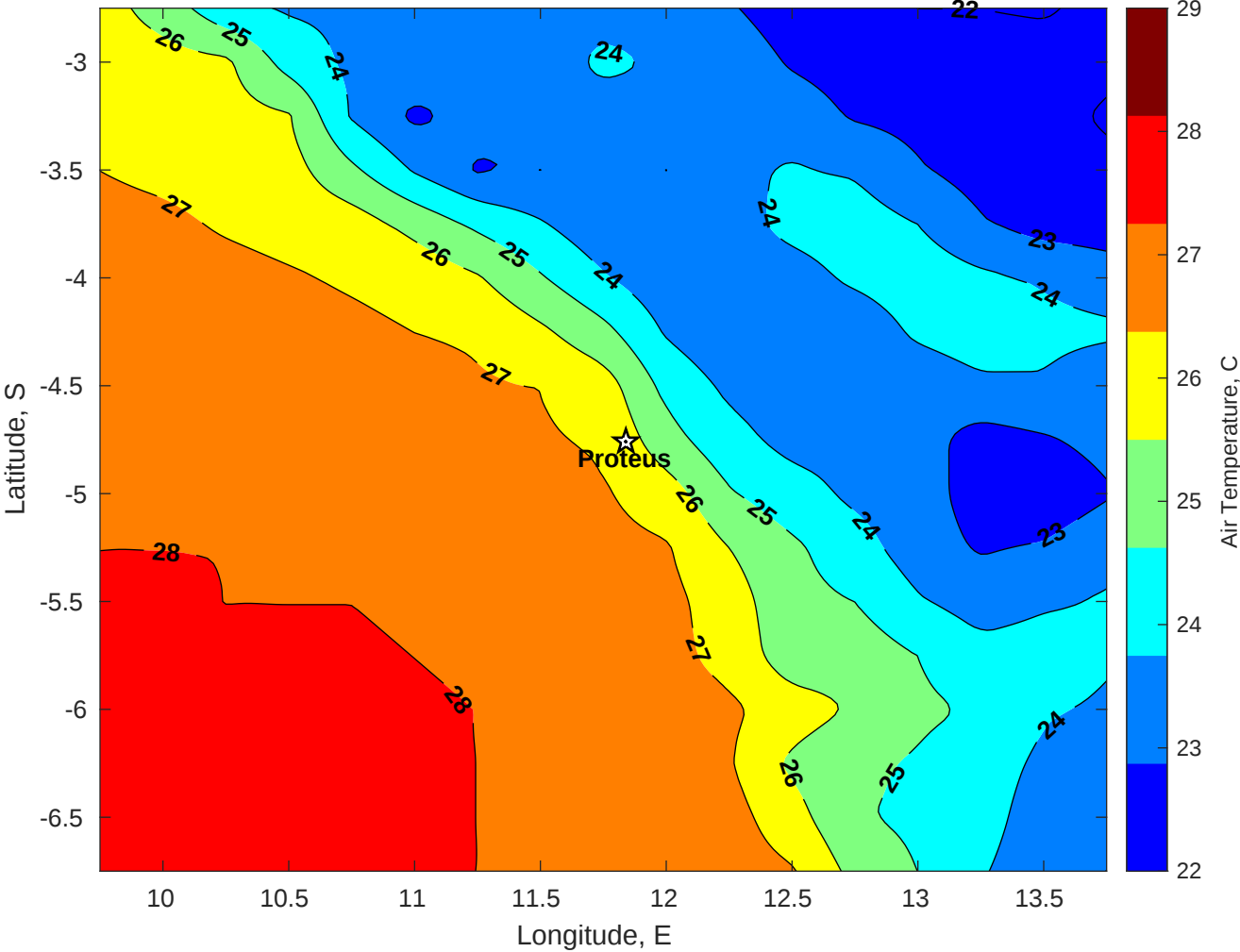
Air Temperature (C) for Proteus at 17-May-2025
