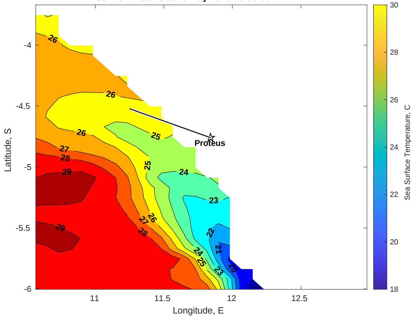
SST for Proteus at 16-May-2025 00:00:00
