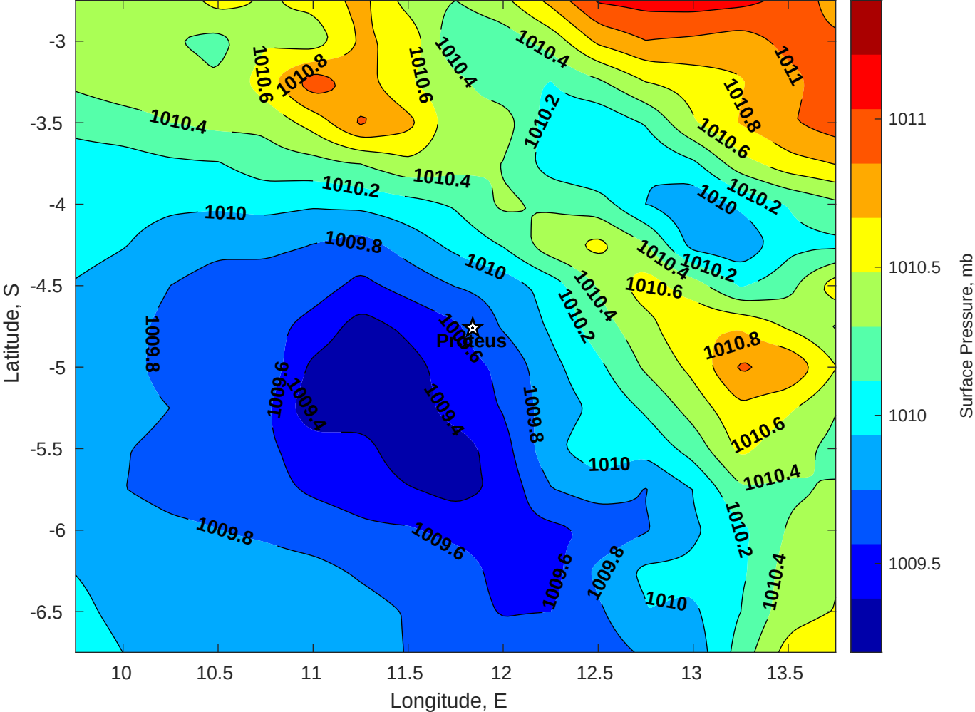
Surface Pressure (mb) for Proteus at 17-May-2025 00:00:00
